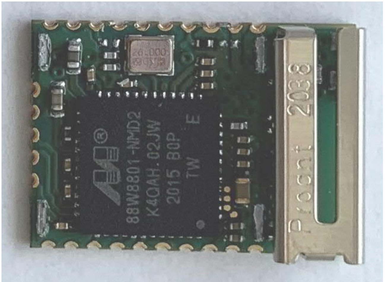
EUT without shieldbox and with antenna (Photo provided by the applicant)
