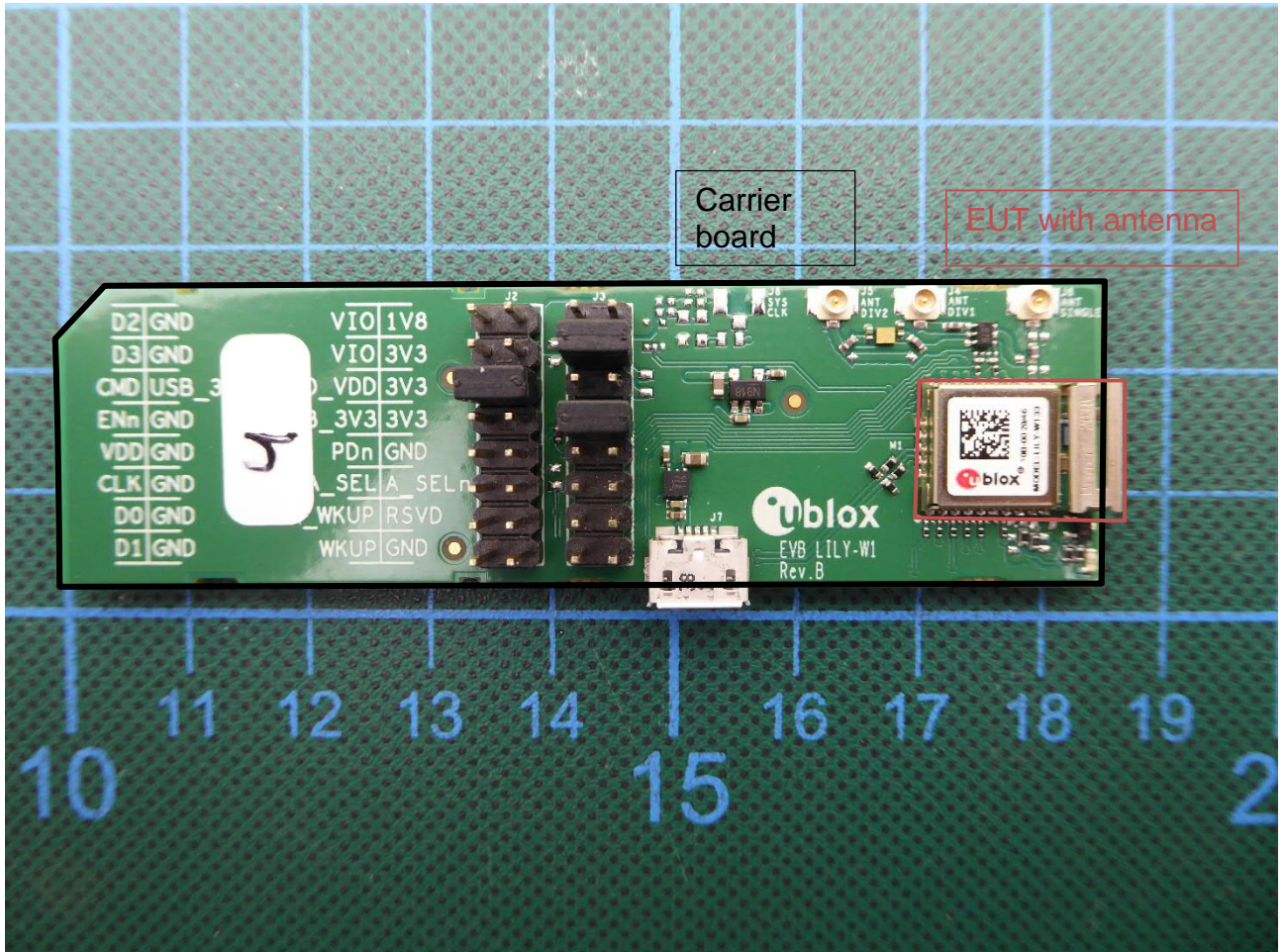
EUT on carrier board
