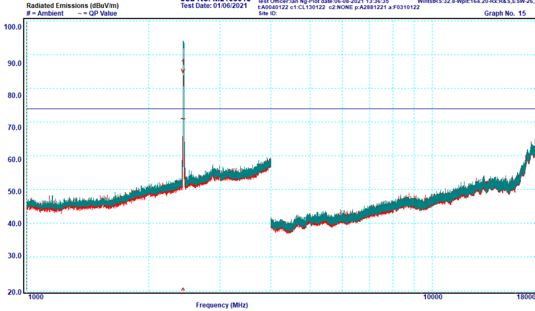
Graph 6-9: Transmitter Spurious Emissions, 1 – 18 GHz, 802.11n 2437 MHz, Peak
