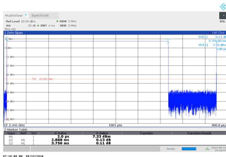
BT Classic DH5 packets
