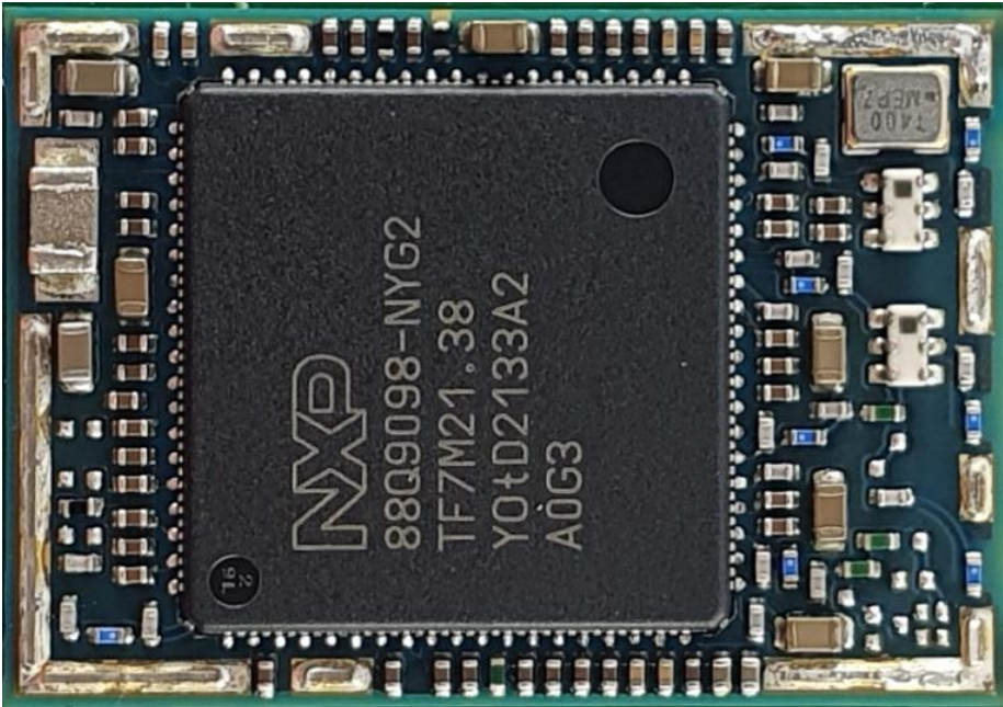
Figure 2: JODY-W377-00B module internal photo
