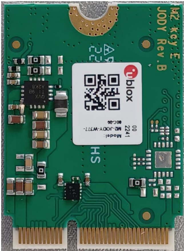
Figure 1: M2-JODY-W377-00B bottom view external photo
