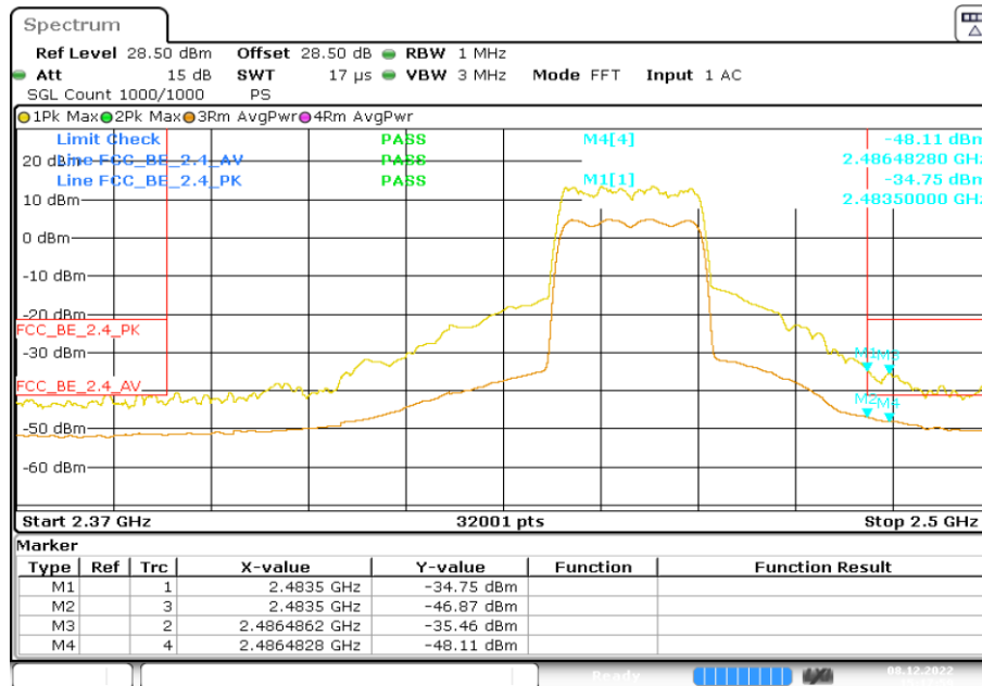
WLAN TX on CH. 9 Ant A
