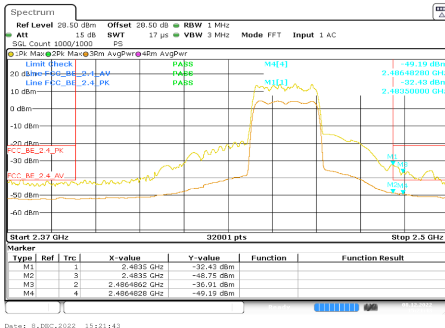
WLAN TX on CH. 9 Ant B
