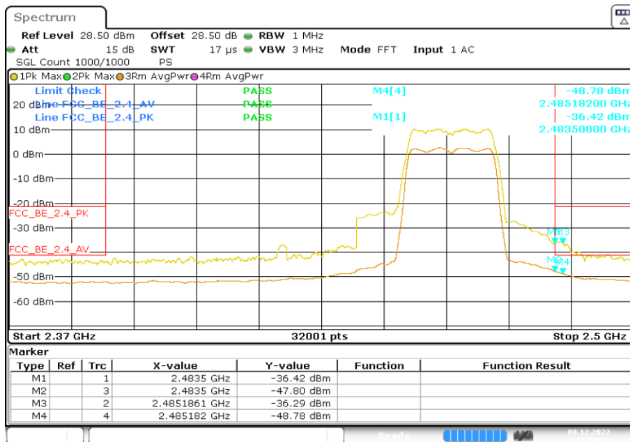
WLAN TX on CH. 11 Ant A
