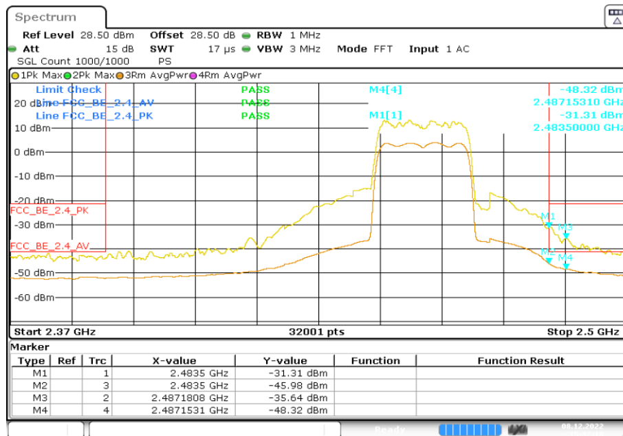
WLAN TX on CH. 10 Ant A
