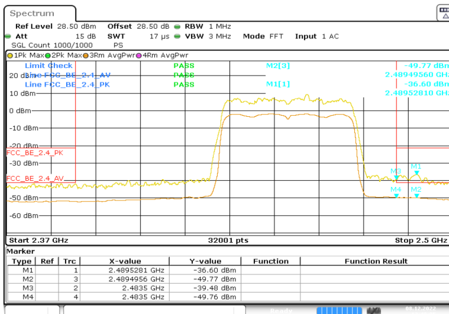
WLAN TX on CH. 9 Ant B
