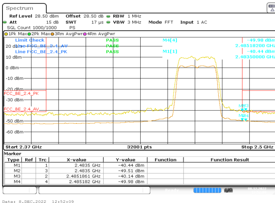
WLAN TX on CH. 11 Ant B
