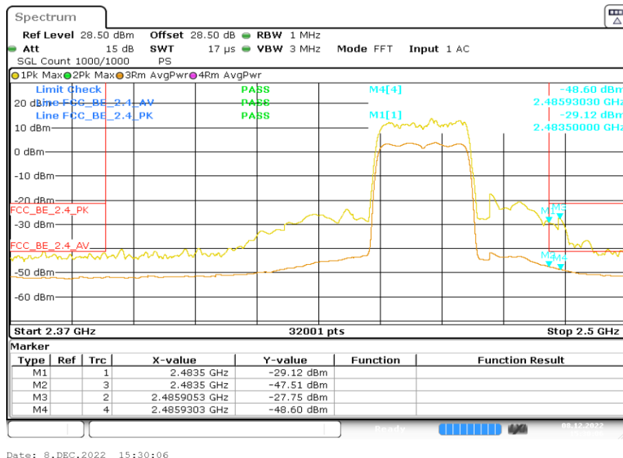
WLAN TX on CH. 10 Ant B
