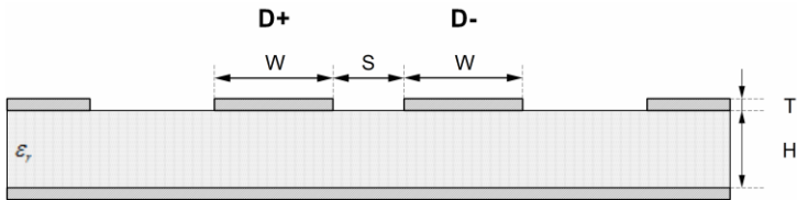
Figure 9: Differential pair, generic controlled impedance parameters
