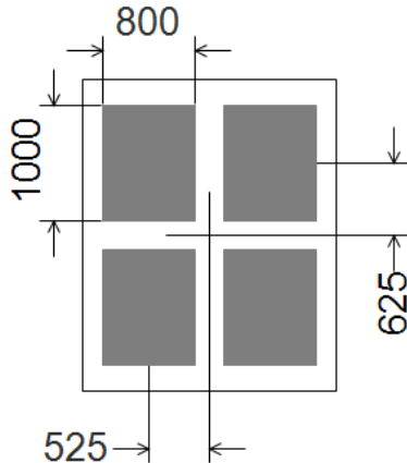
Figure 12: Stencil opening example for inner thermal pads (dimensions in μm)
