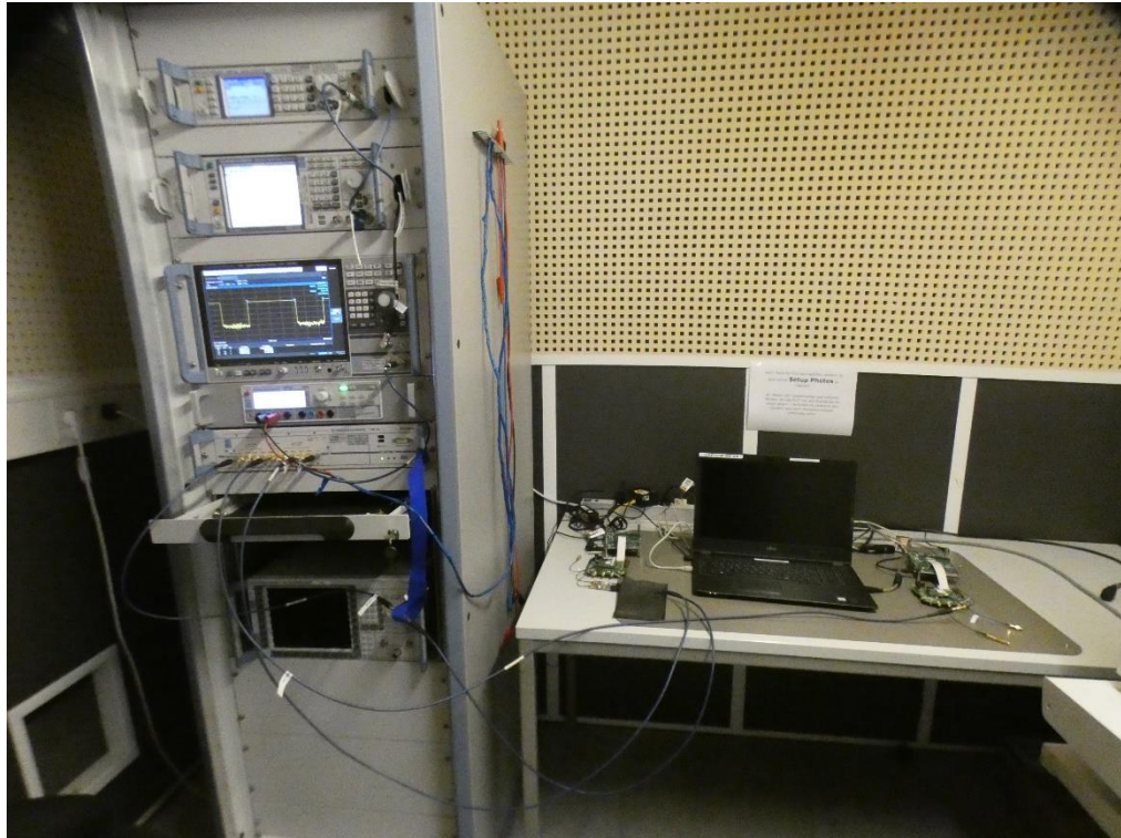
Photo 1: Test setup for conducted DFS tests
