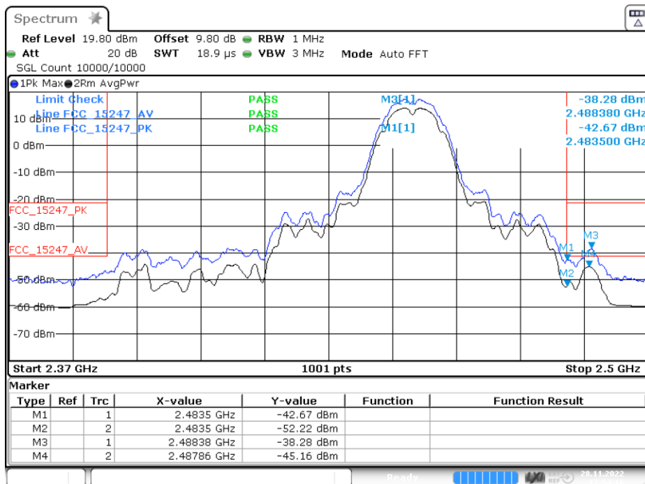
Channel 9 at power setting 21 dBm
