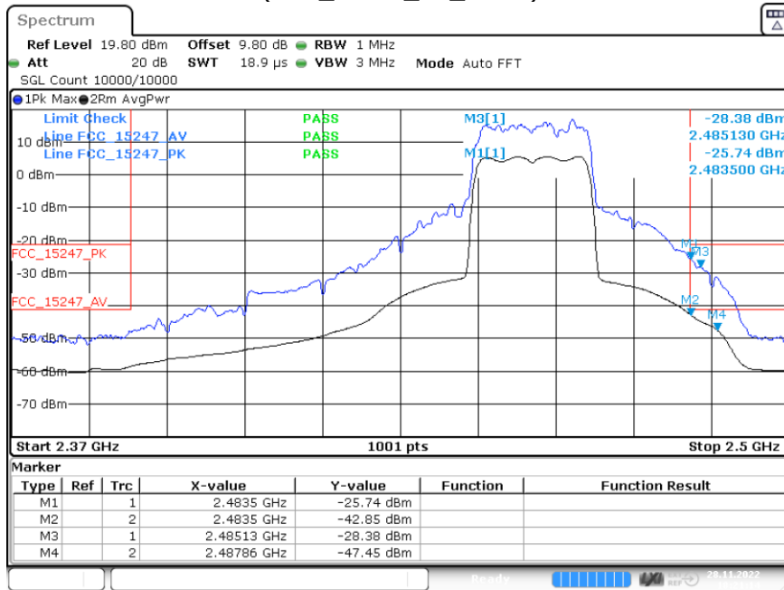
Channel 10 at power setting 14 dBm
