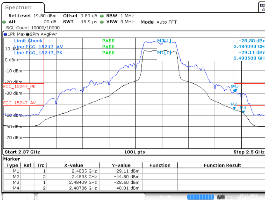
Channel 9 at power setting 16 dBm
