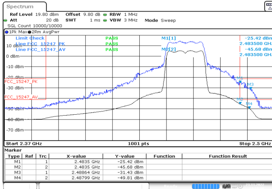
Channel 10 at power setting 14 dBm
