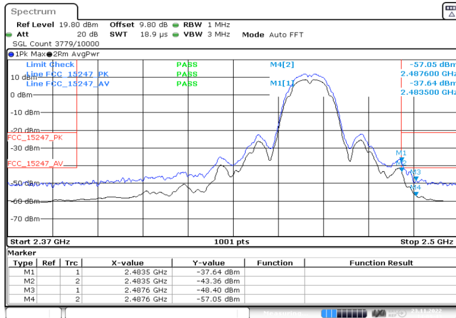
Channel 10 at power setting 16 dBm
