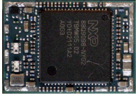
Figure 2: JODY-W374-20A internal photo
