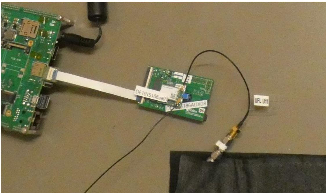
Photo 6: Test setup for conducted measurements EUT Detail
