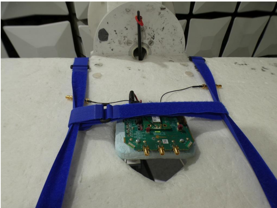
Photo 4: Test setup for radiated measurements above 1 GHz EUT Detail
