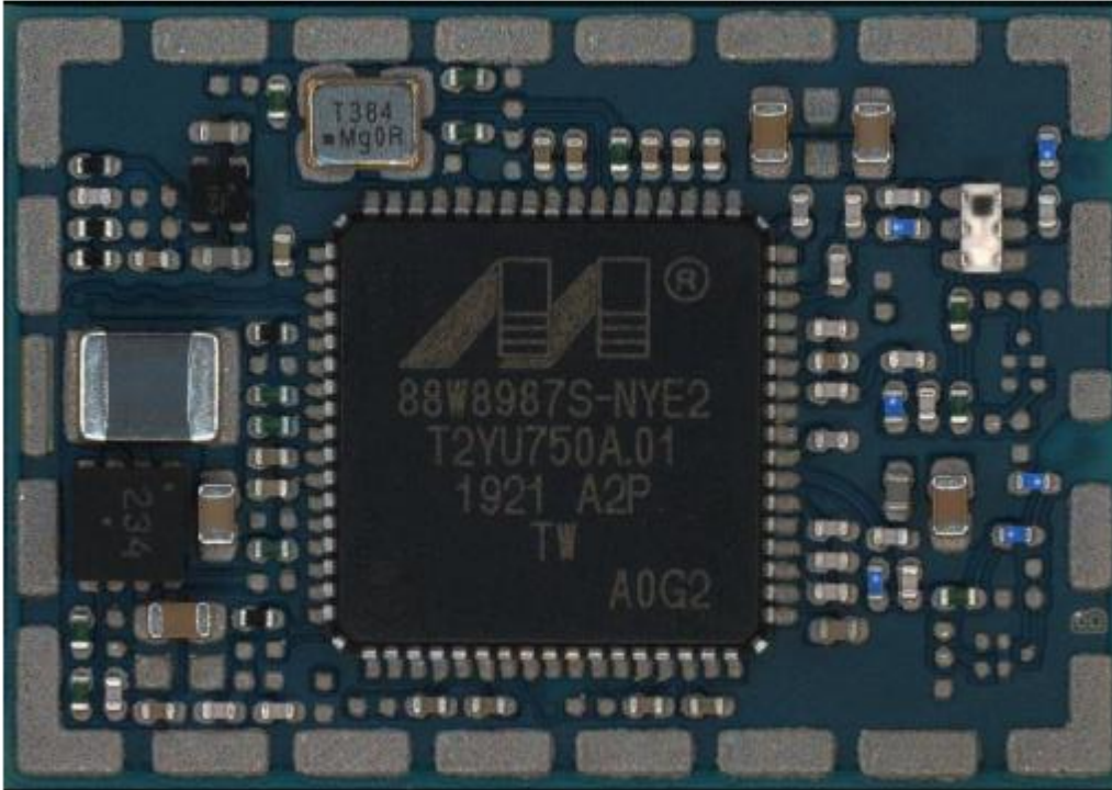
Figure 1: JODY-W263-01A, JODY-W263-00A and JODY-W263-00B internal photo
