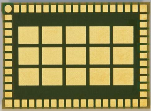
Figure 8: Bottom view for all module variants
