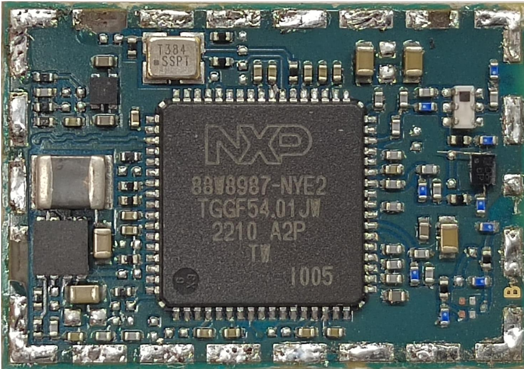
Figure 2: JODY-W263-01B, JODY-W263-11B and JODY-W263-10A internal photo
