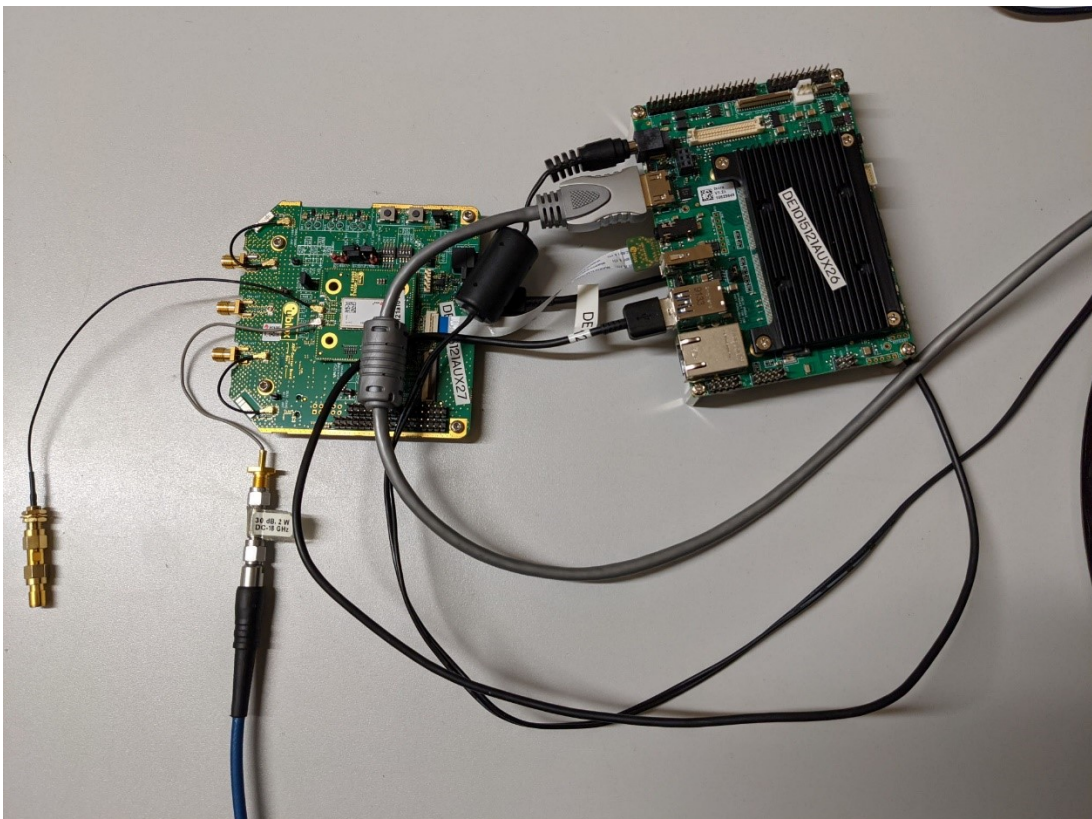
Photo 8: Test Setup for DFS (Client Detail)
