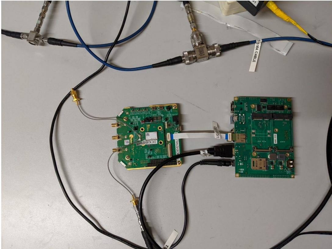
Photo 8: Test Setup for DFS (Master Detail)
