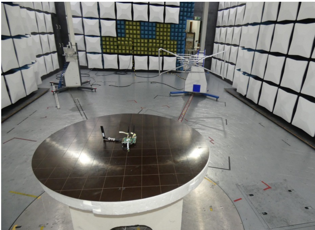
Photo 2: Test setup for radiated measurements below 1 GHz
