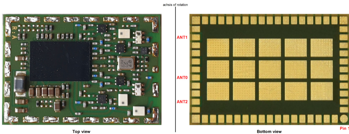
Figure 1: JODY-W167-00A, JODY-W167-03A and JODY-W167-00B internal photo (Top view) with marked antenna pins (Bottom view)
