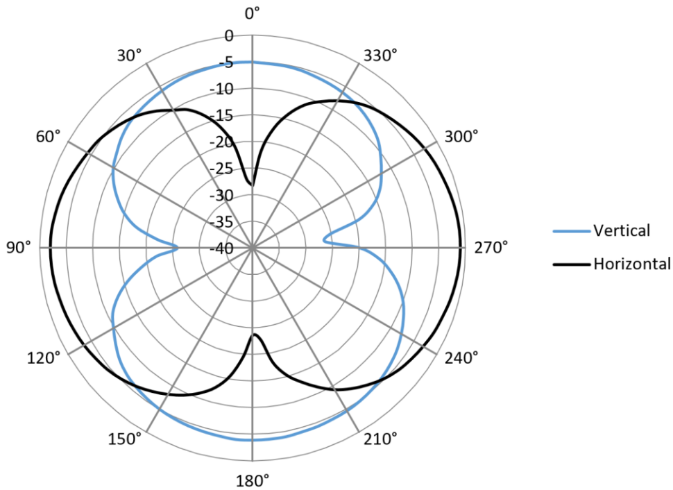
Figure 15: Y-Z plane antenna pattern
