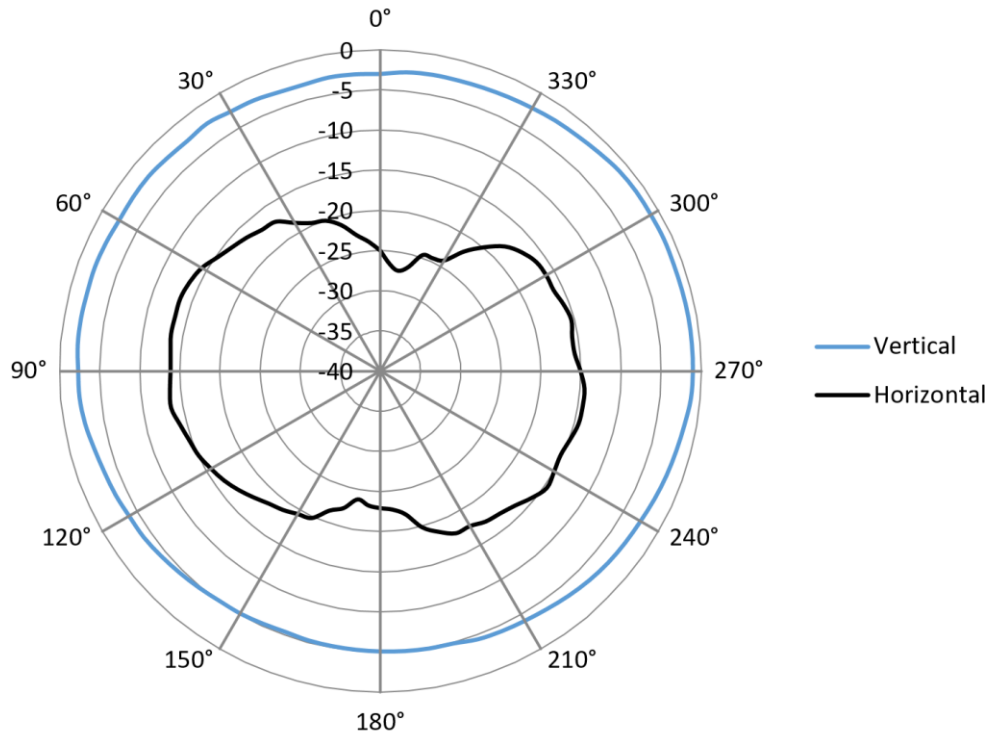
Figure 13: X-Y plane antenna pattern
