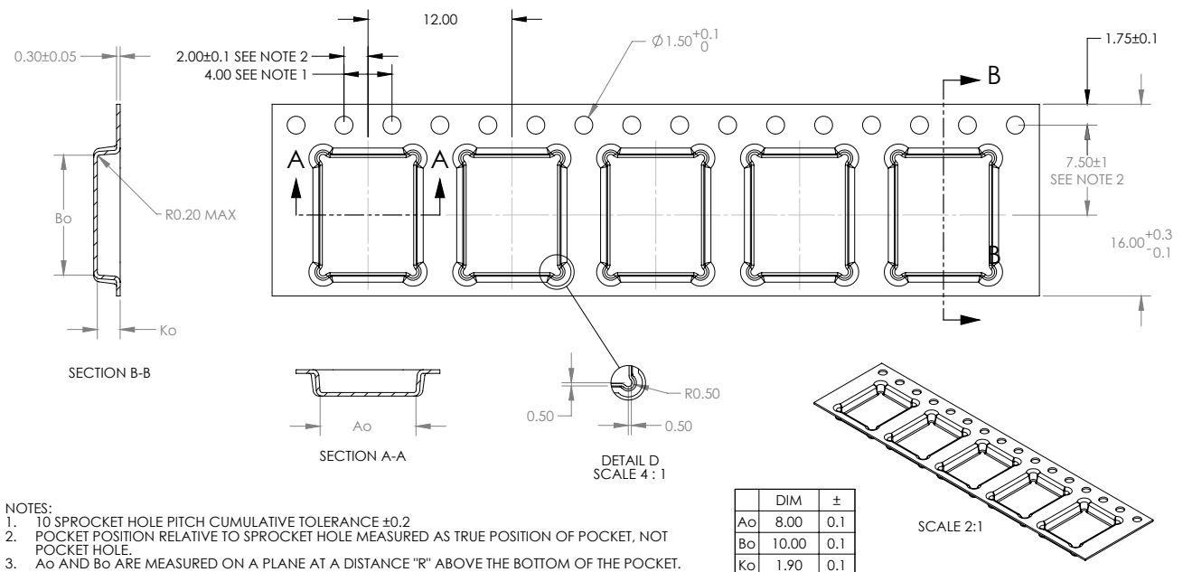
Figure 17 – Carrier tape dimensions for type number BMD-380-A-R-10
