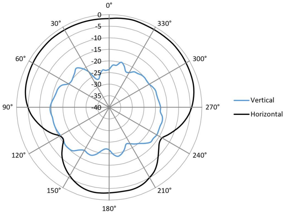
Figure 14: X-Z plane antenna pattern
