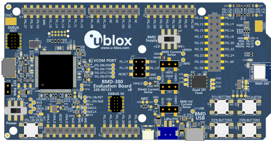
Figure 16: BMD-380 evaluation board
