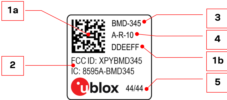
Figure 6: Module marking
