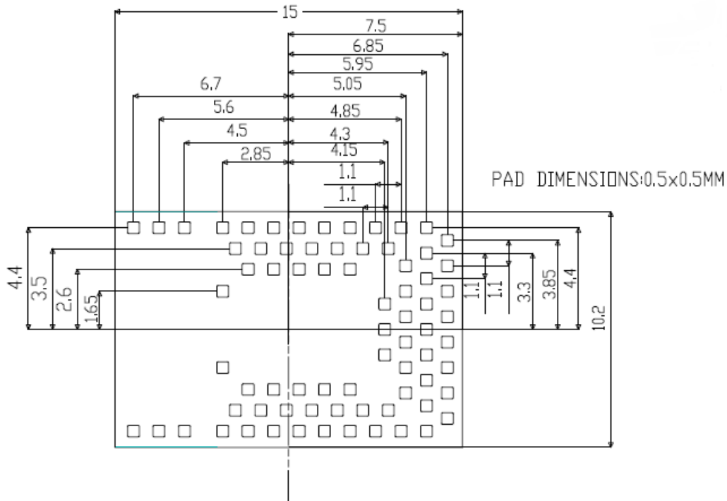
Figure 5: Recommended PCB land pads (dimensions in mm)
