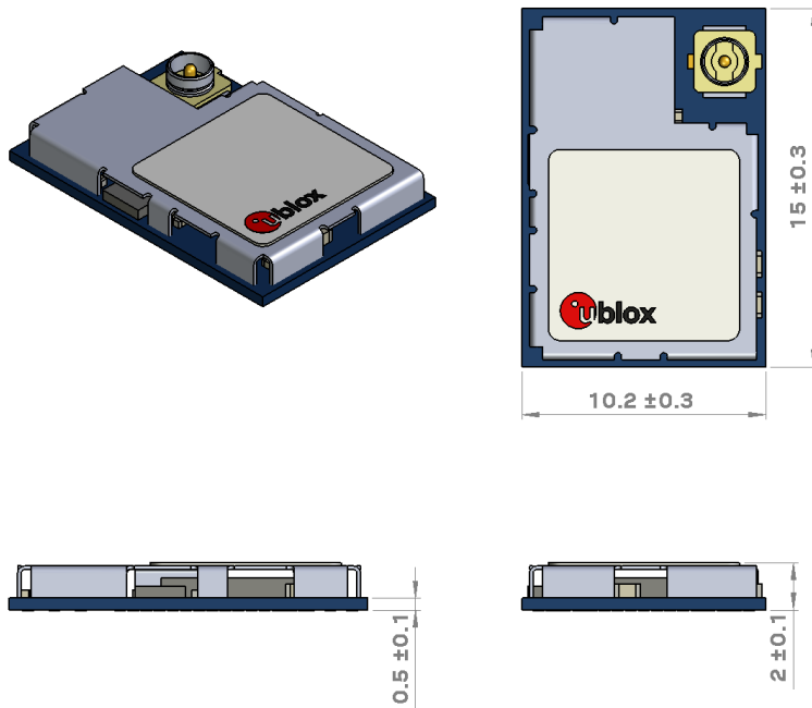
Figure 4: BMD-345 mechanical drawing (dimensions in mm)
