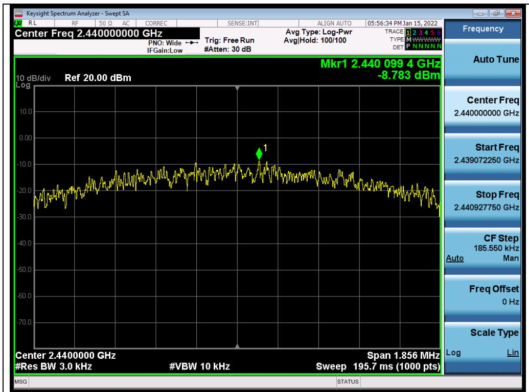
Test_Graph_LE2M_ANT1_2440_2Mbps_PSD
