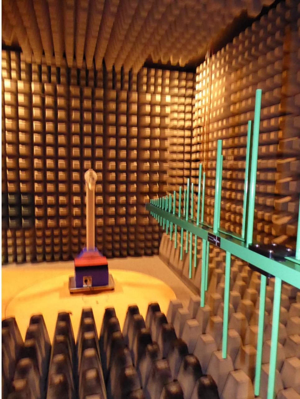
181323_SetRadU8.JPG: Test setup fully anechoic chamber; EVB-ANNA-B112U#117, 30 MHz – 1 GHz
