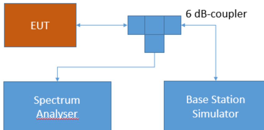
Test Setup FCC Part 22/24/27/90 Cellular;
