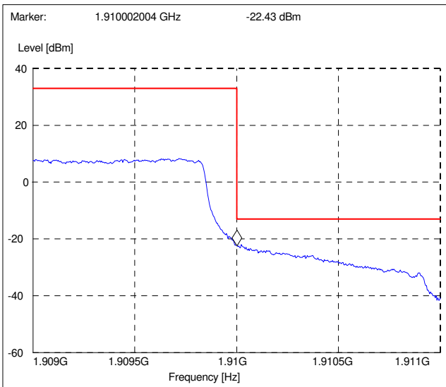
1909.3 MHz, QPSK, 6RB, RMS, RBW = 20kHz
