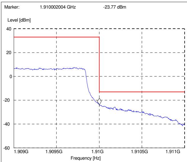
1909.3 MHz, 16QAM, 6RB, RMS, RBW = 20kHz
