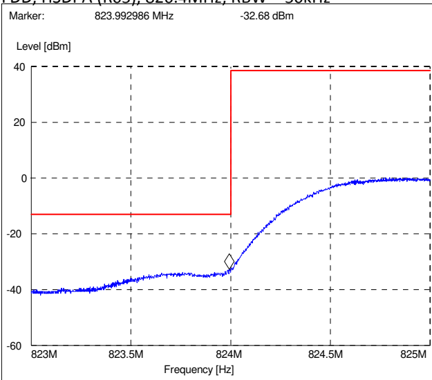
FDD, HSDPA (R05), 826.4MHz, RBW = 50kHz
