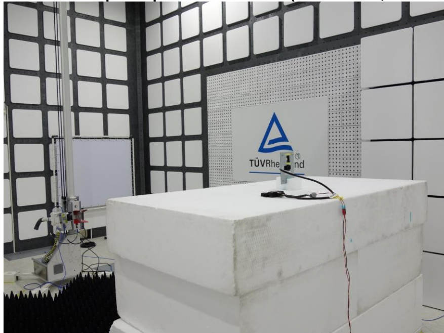
Photograph 12: Test Setup for Spurious Emissions (Back View 2, GSM850)
