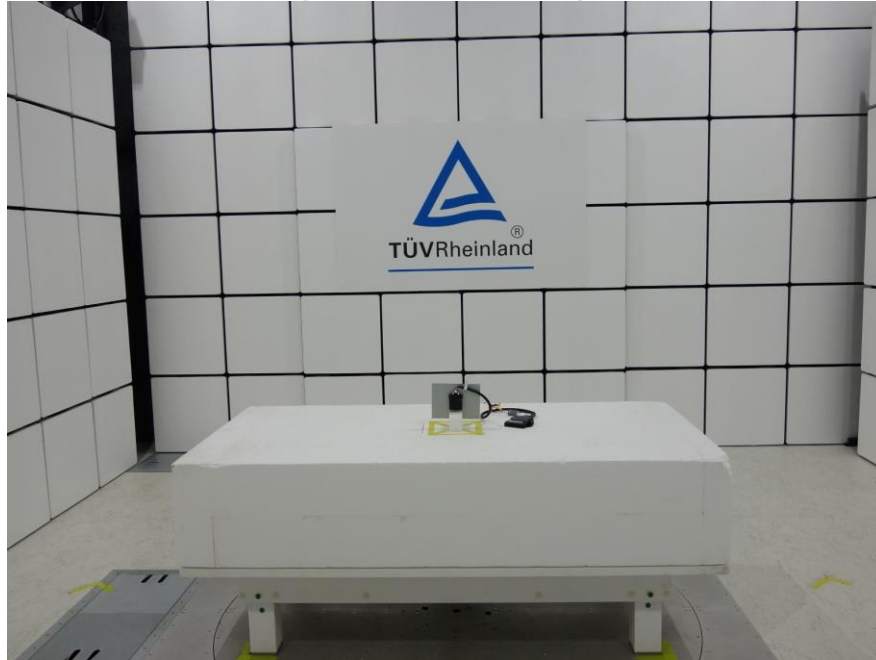
Photograph 14: Test Setup for Spurious Emissions (Front View 2, GSM1900)
