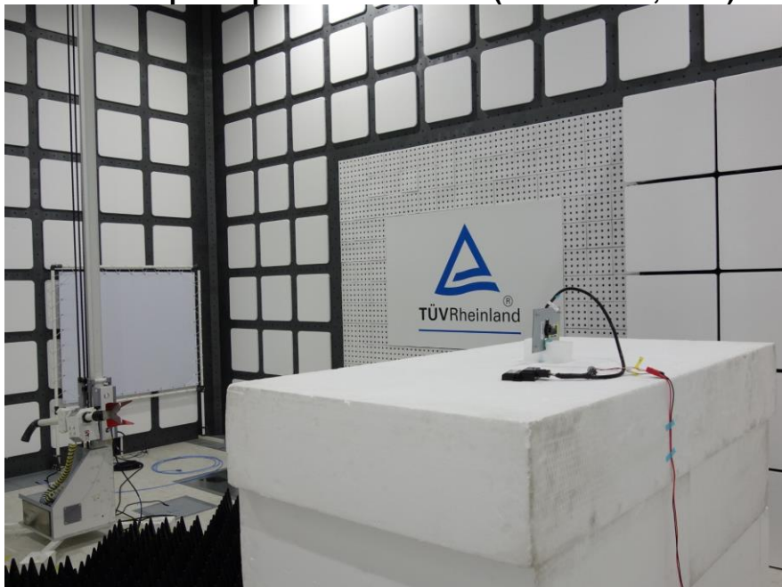
Photograph 4: Test Setup for Spurious Emissions (Back View 2, GSM)
