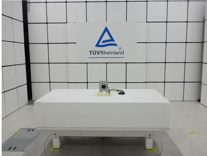
Photograph 22: Test Setup for Spurious Emissions (Front View 2, WCDMA Band V)
