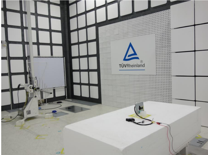
Photograph 3: Test Setup for Spurious Emissions (Back View 1, GSM)
