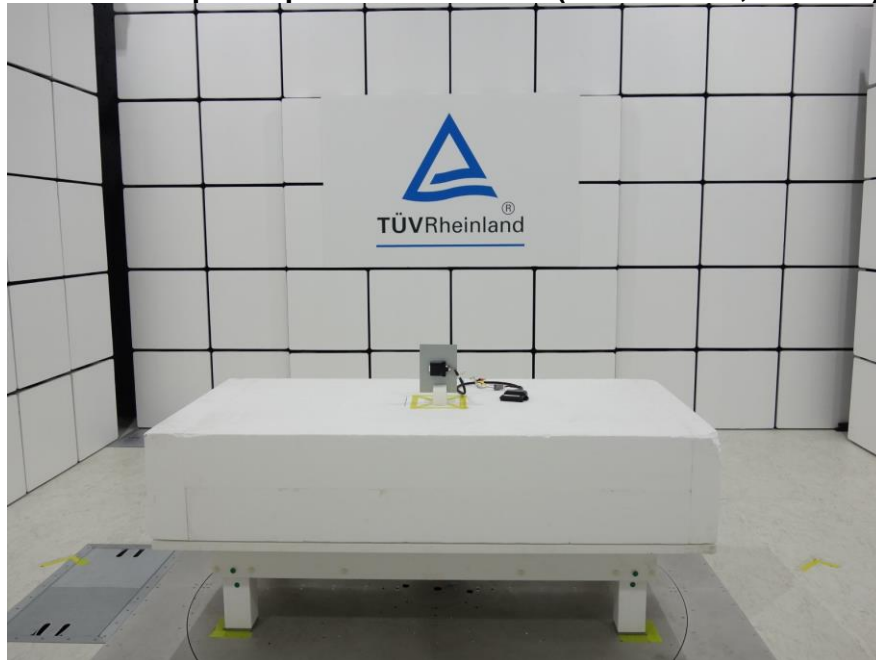
Photograph 10: Test Setup for Spurious Emissions (Front View 2, GSM850)
