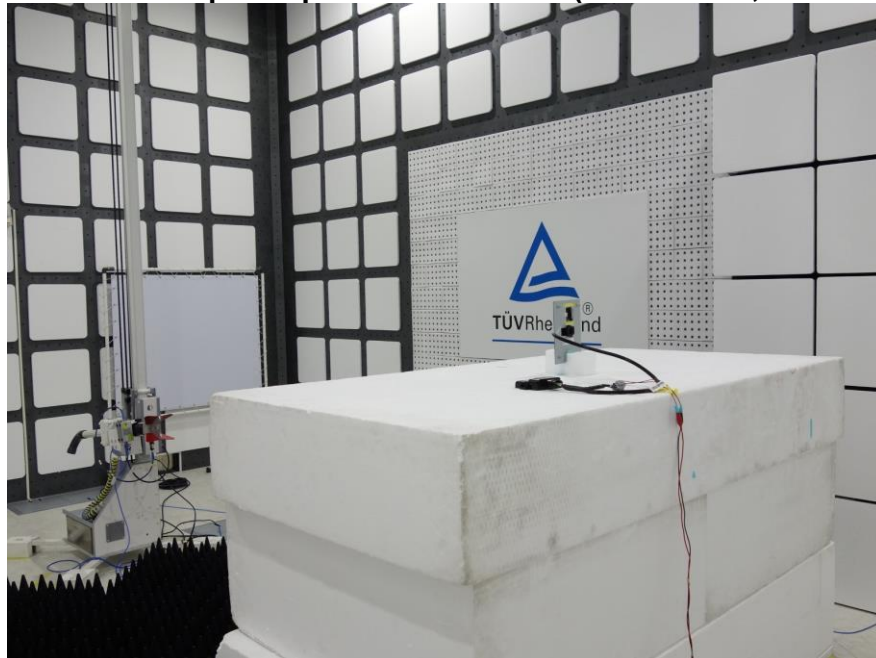
Photograph 24: Test Setup for Spurious Emissions (Back View 2, WCDMA Band V)
