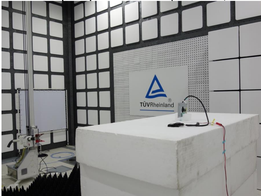
Photograph 16: Test Setup for Spurious Emissions (Back View 2, GSM1900)
