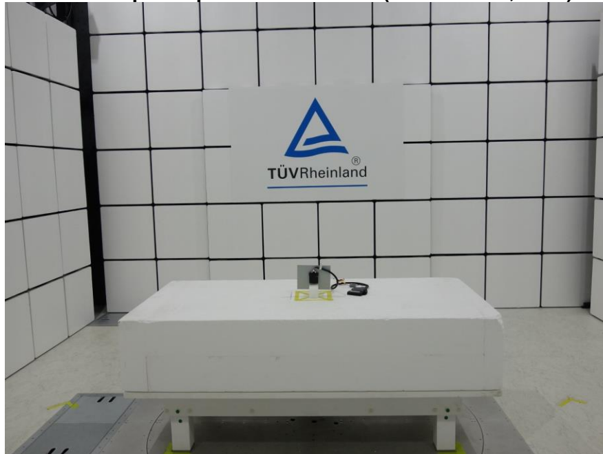
Photograph 2: Test Setup for Spurious Emissions (Front View 2, GSM)
