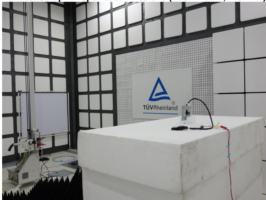
Photograph 8: Test Setup for Spurious Emissions (Back View 2, WCDMA)
