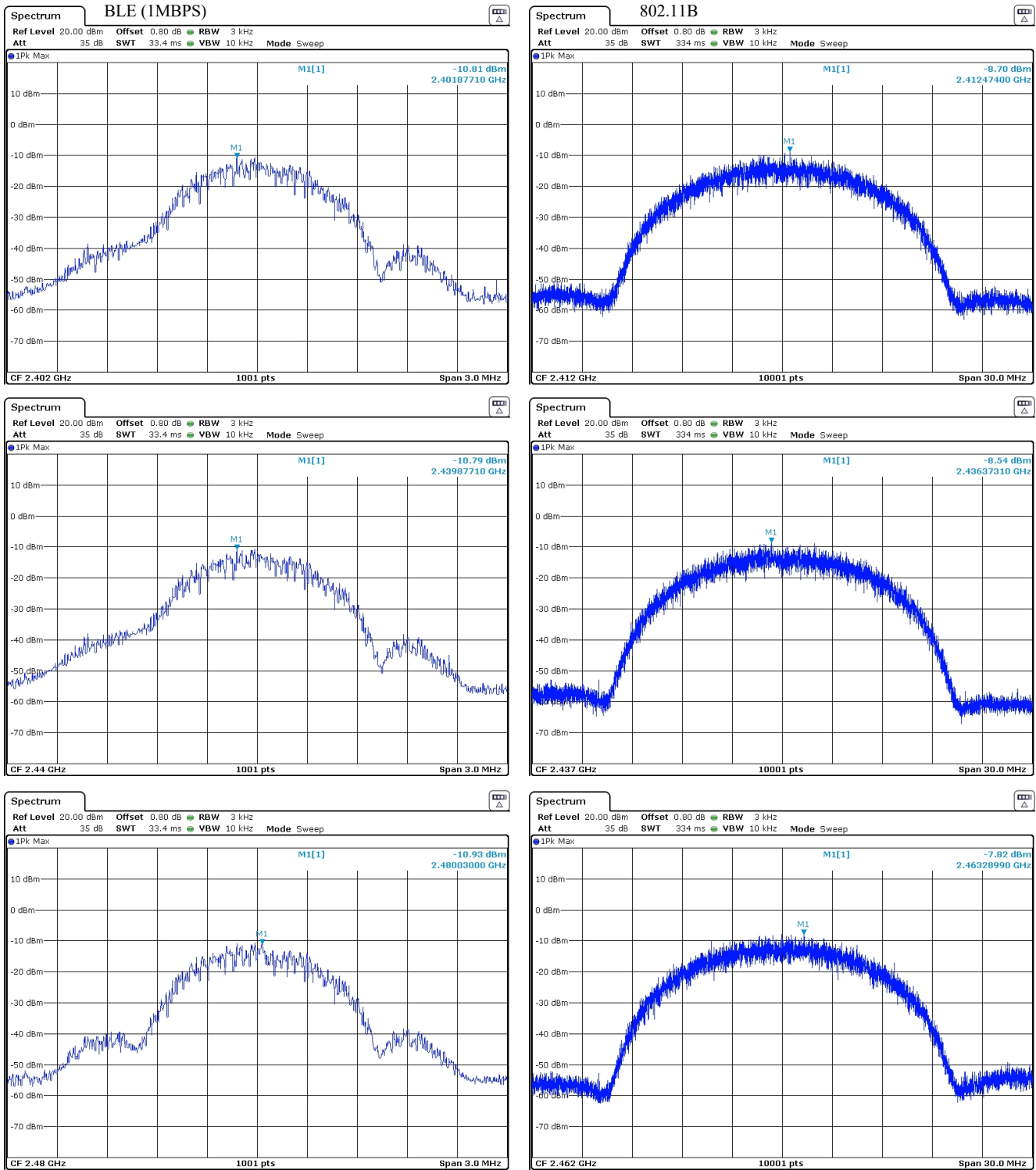
Figure 9(a): Power Spectral Density Plots.
