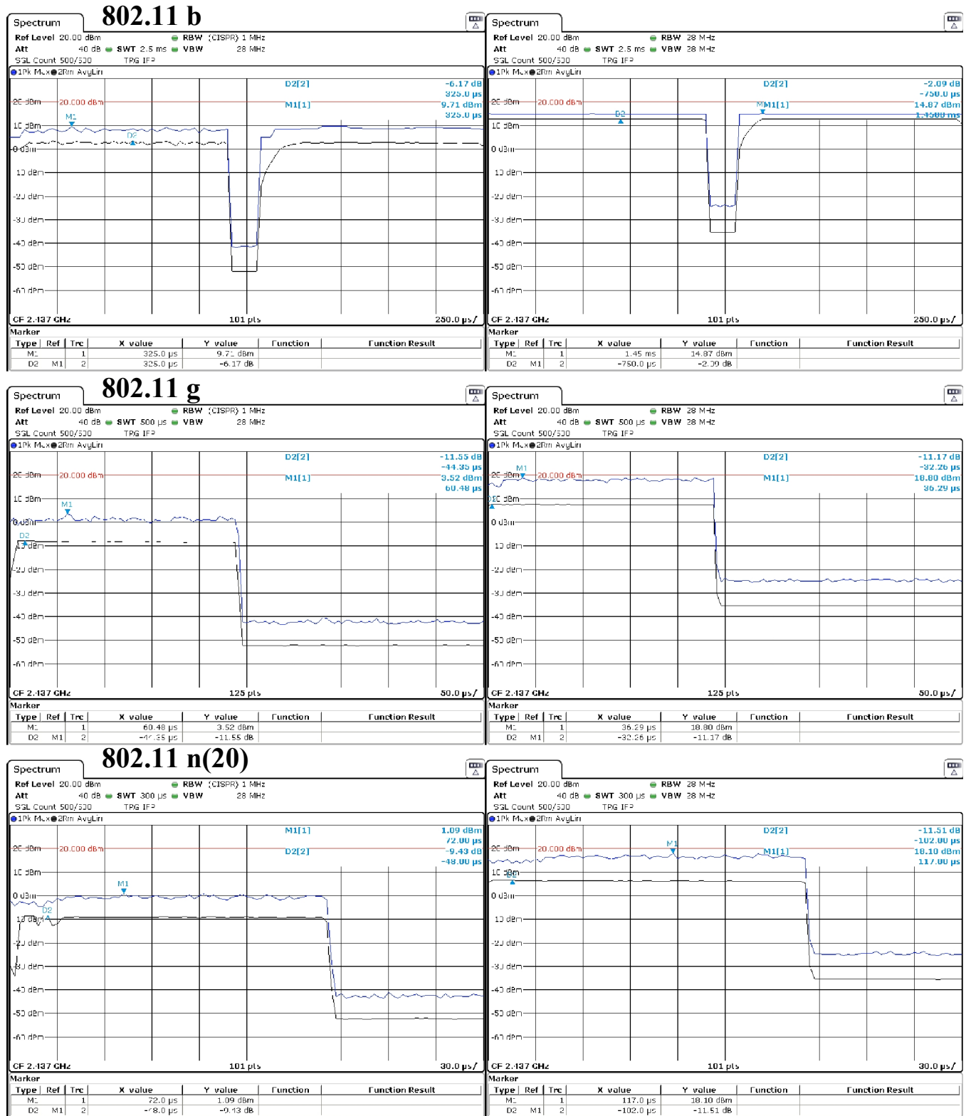
Figure 6(a): Pulsed Emission Characteristics (Duty Cycle).
