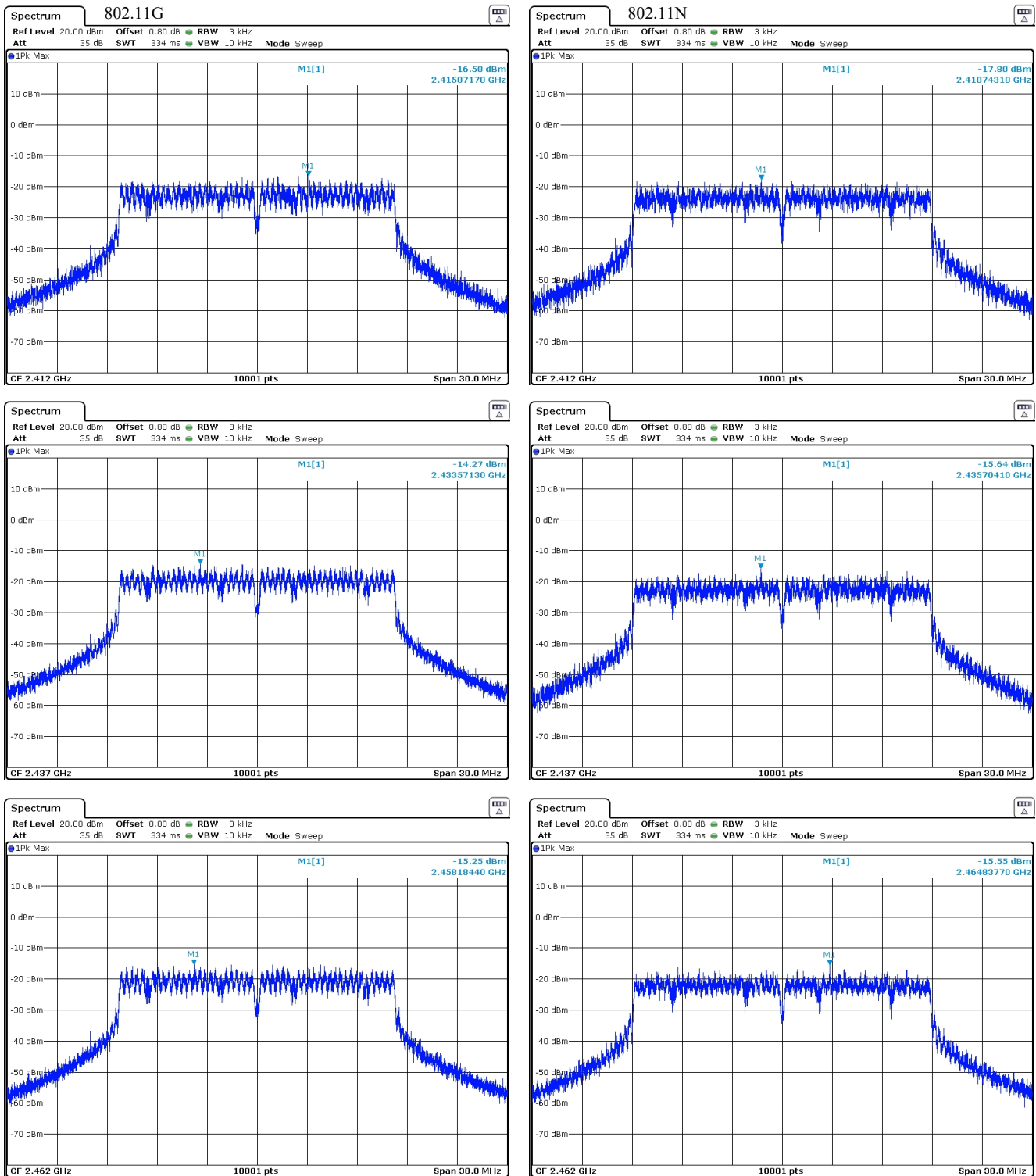
Figure 9(b): Power Spectral Density Plots.
