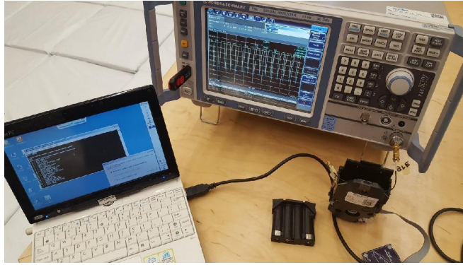
Figure 5: Conducted RF Test Setup Photograph(s).
