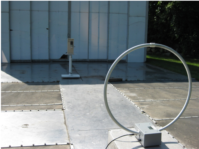
Setup of EUT on the 10m OATS
