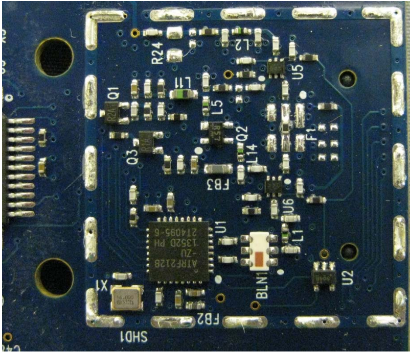
Close Up of RF Section
