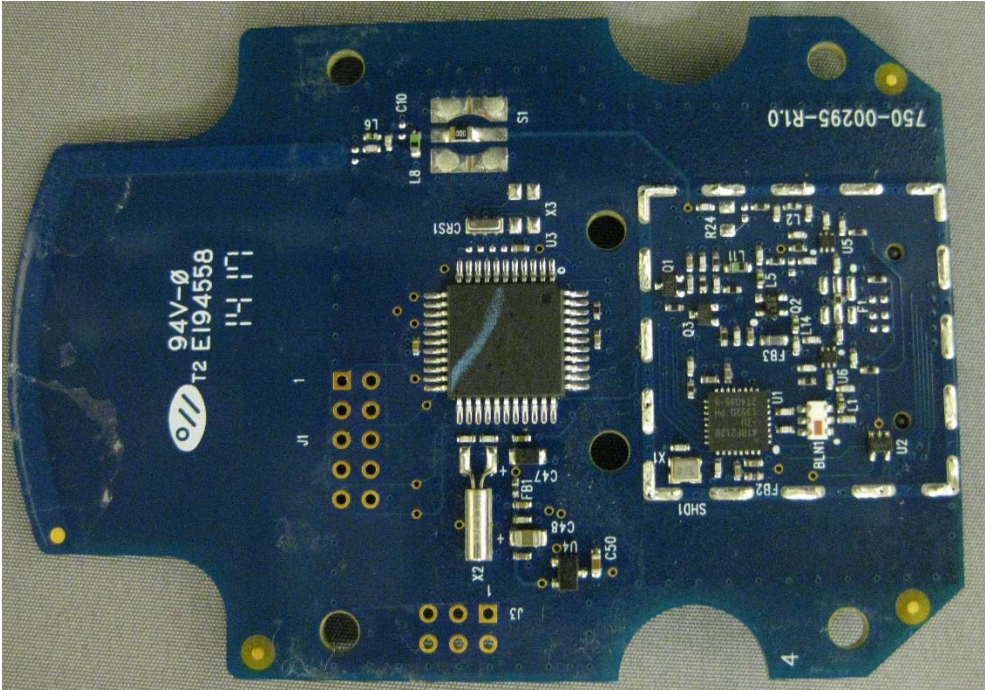
Shield Removed
