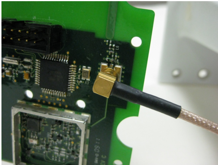
Close Up of Module with Antenna Connection
