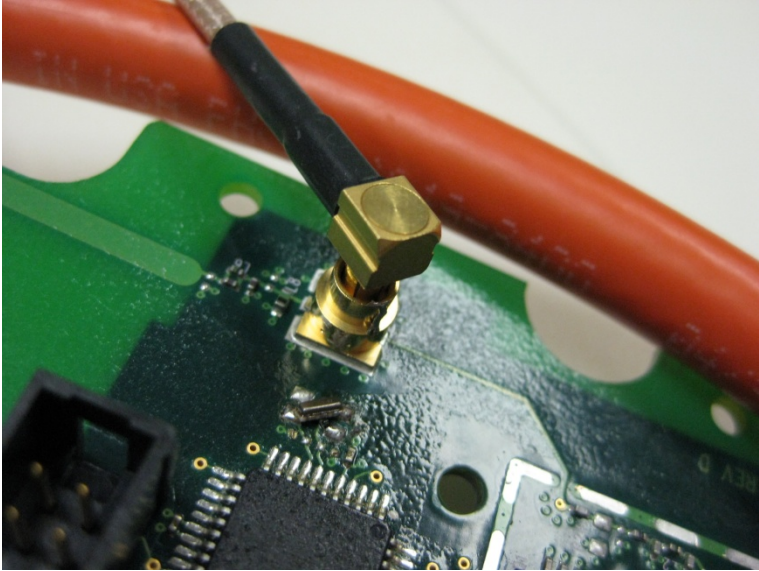
Antenna Connected
