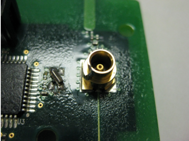
Close Up of Antenna Connector
