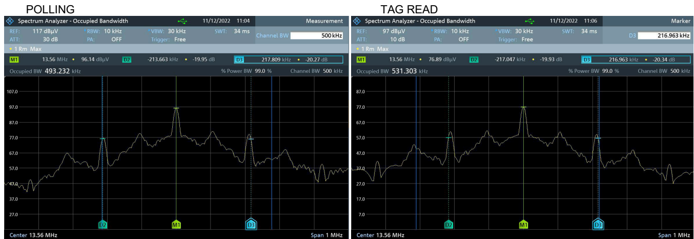
Figure 8: Example Intentional Emission Bandwidth.
