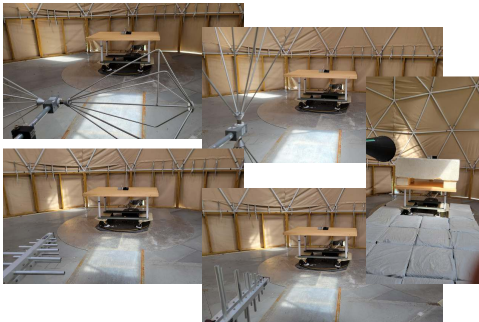
Figure 4.1.1 (iv) Radiated Emissions Test Setup Photograph(s).
