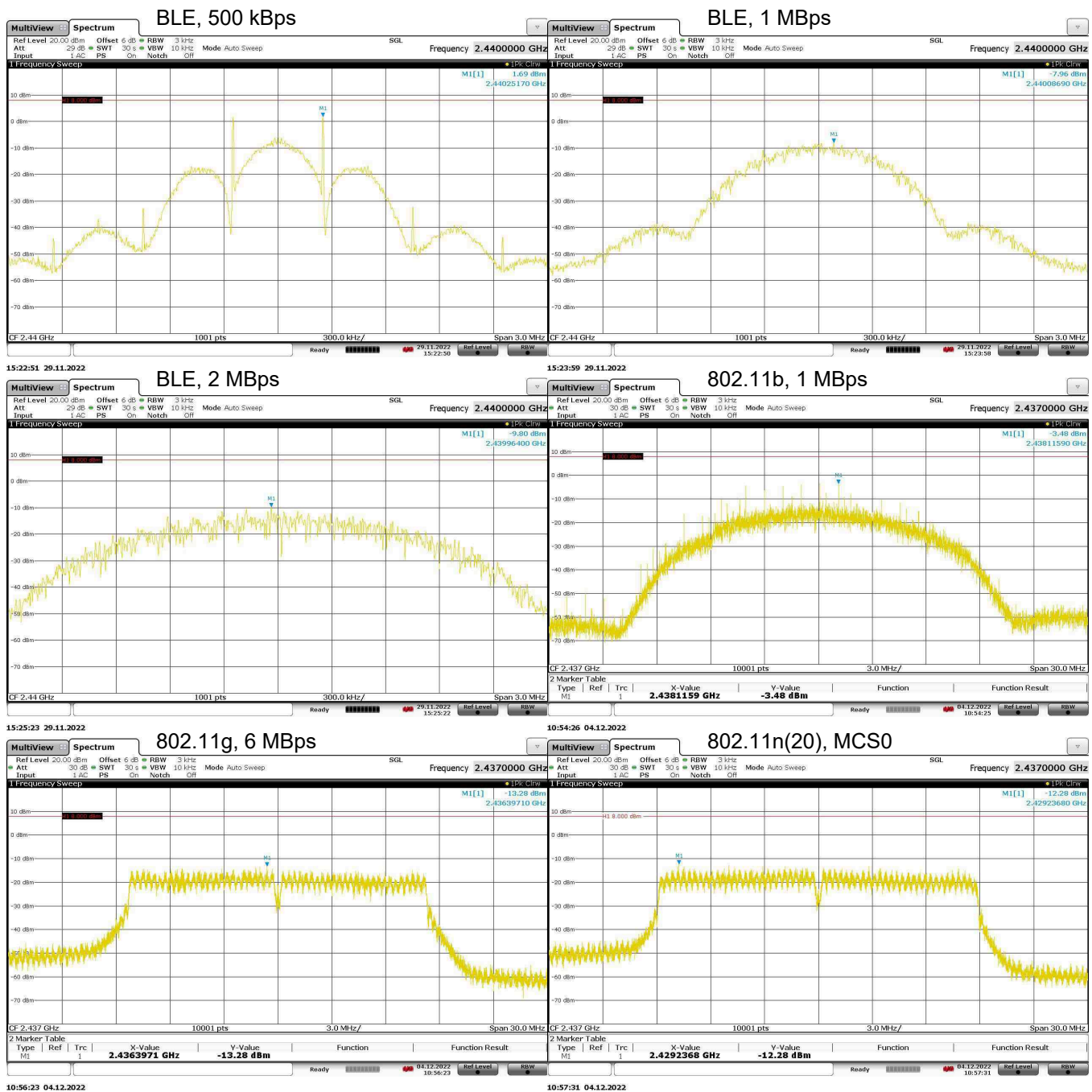
Figure 10: Power Spectral Density Plots.
