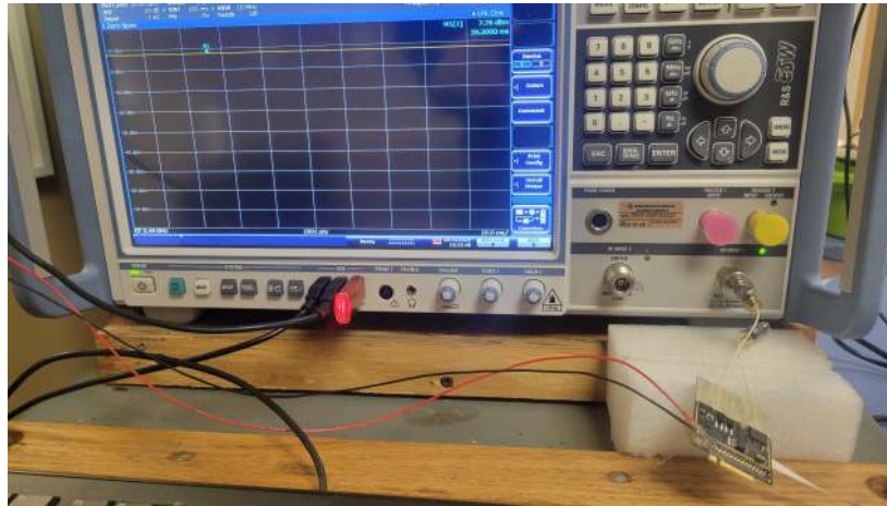
Figure 5: Conducted RF Test Setup Photograph(s).
