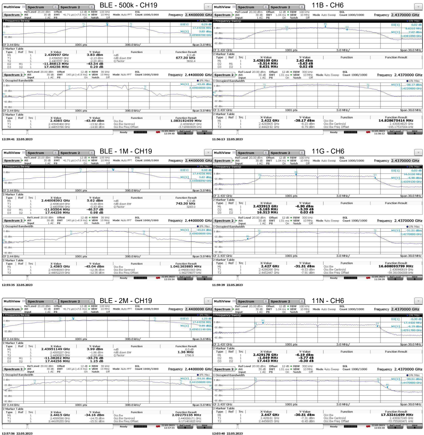
Figure 9: Example Intentional Emission Bandwidth Plots.
