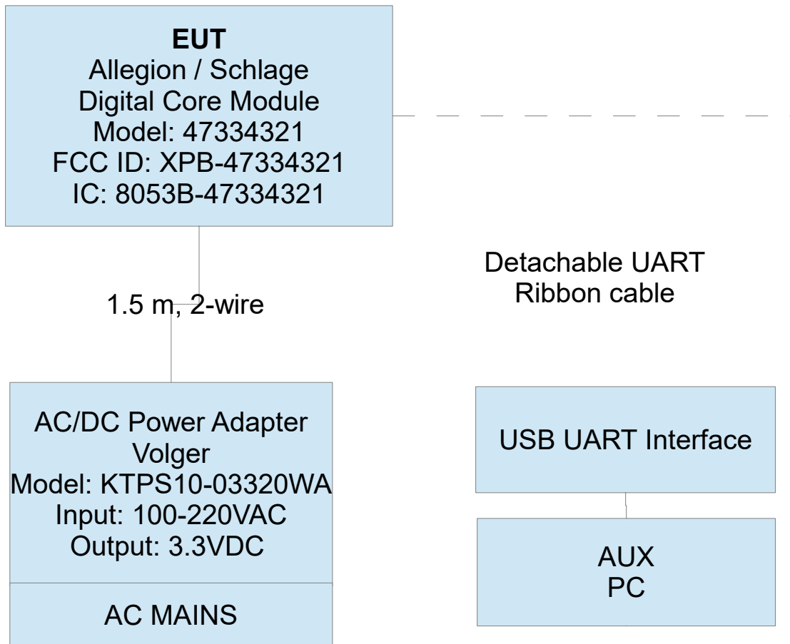
Figure 2: EUT Test Configuration Diagram.
