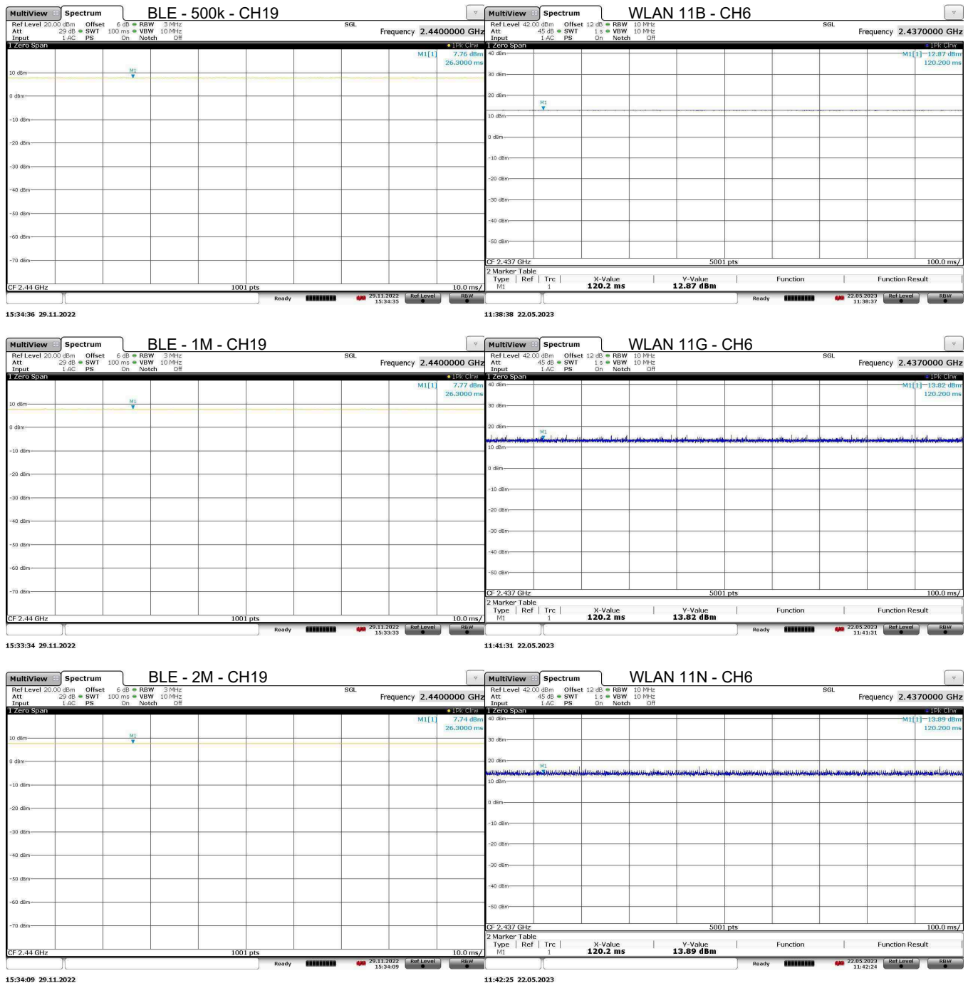
Figure 8: Example Pulsed Emission Characteristics (Duty Cycle).
