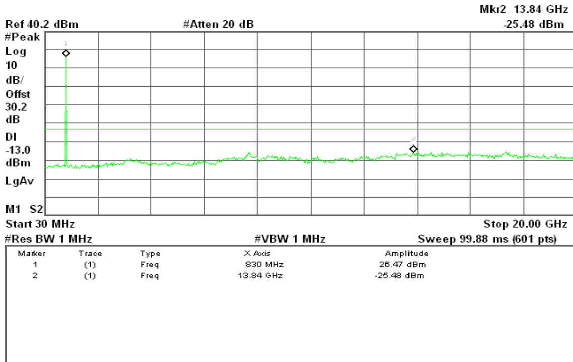
Figure 8-3: Out of Band emission at antenna terminals – CDMA2000 1xEVDO / CH High
