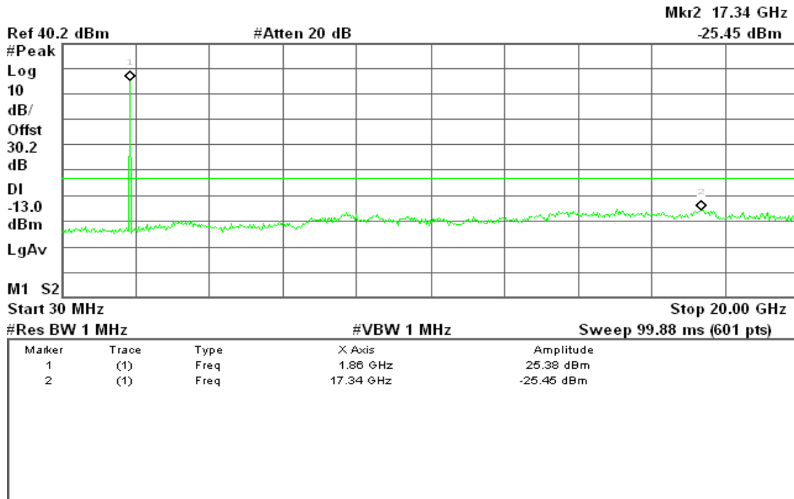
Figure 10-1: Out of Band emission at antenna terminals – CDMA2000 1xEVDO / CH Low
