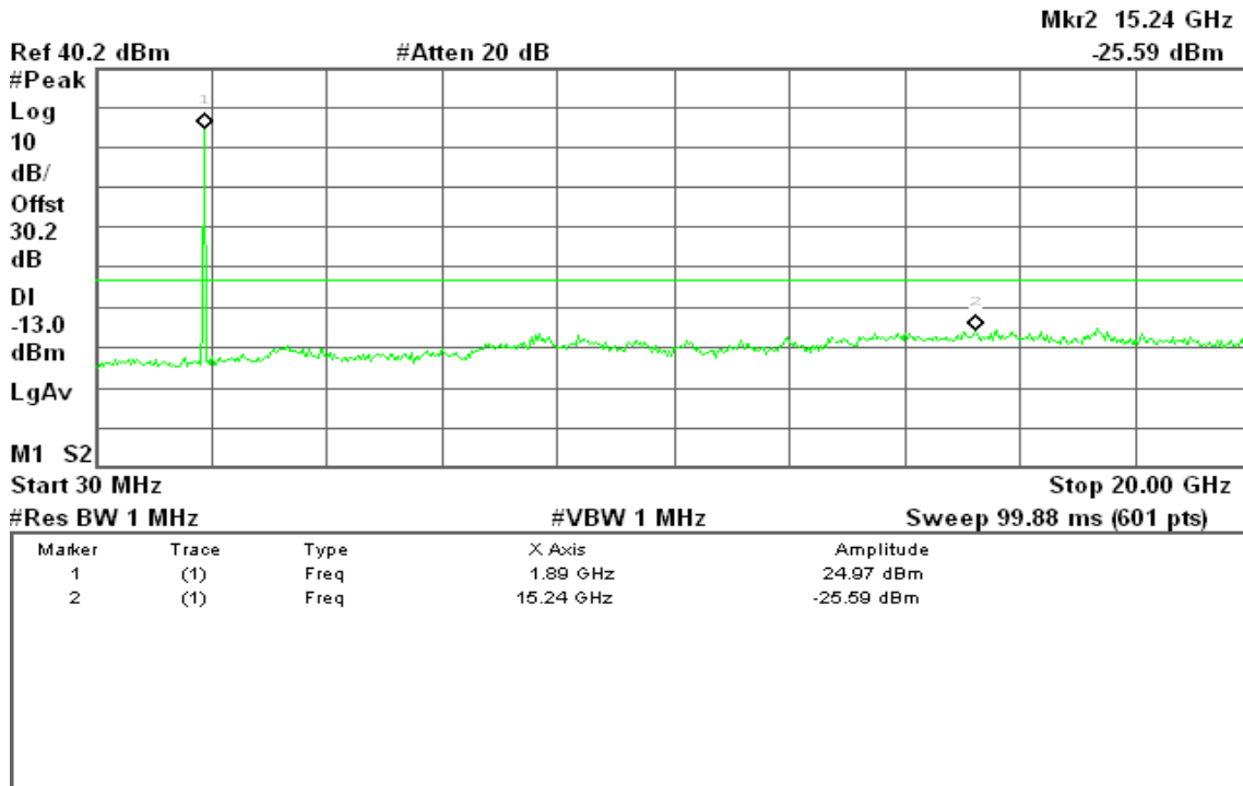
Figure 10-3: Out of Band emission at antenna terminals – CDMA2000 1xEVDO / CH High
