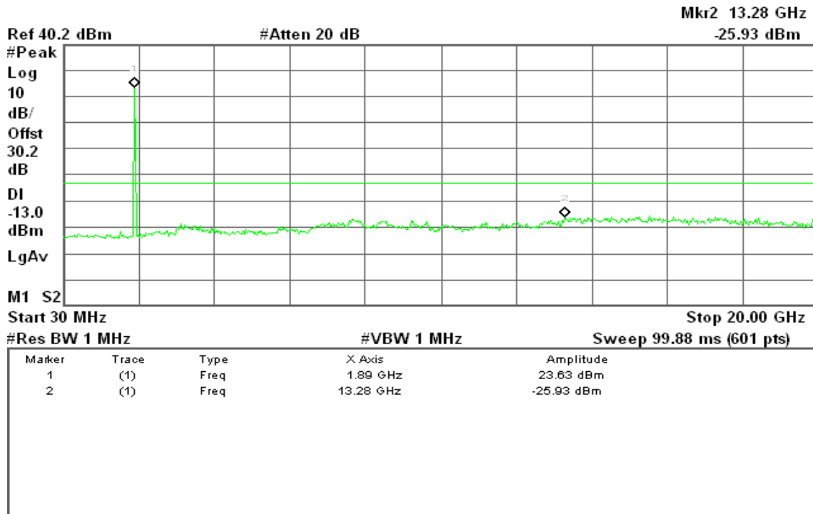
Figure 9-3: Out of Band emission at antenna terminals – CDMA2000 1xRTT / CH High
