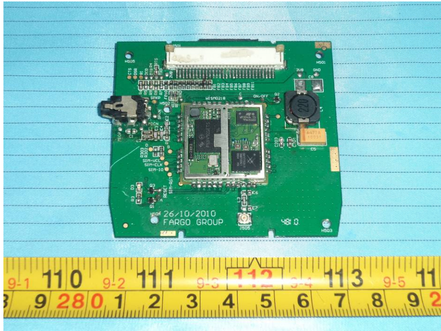
EUT – RF Module Board Shielding off Top View
