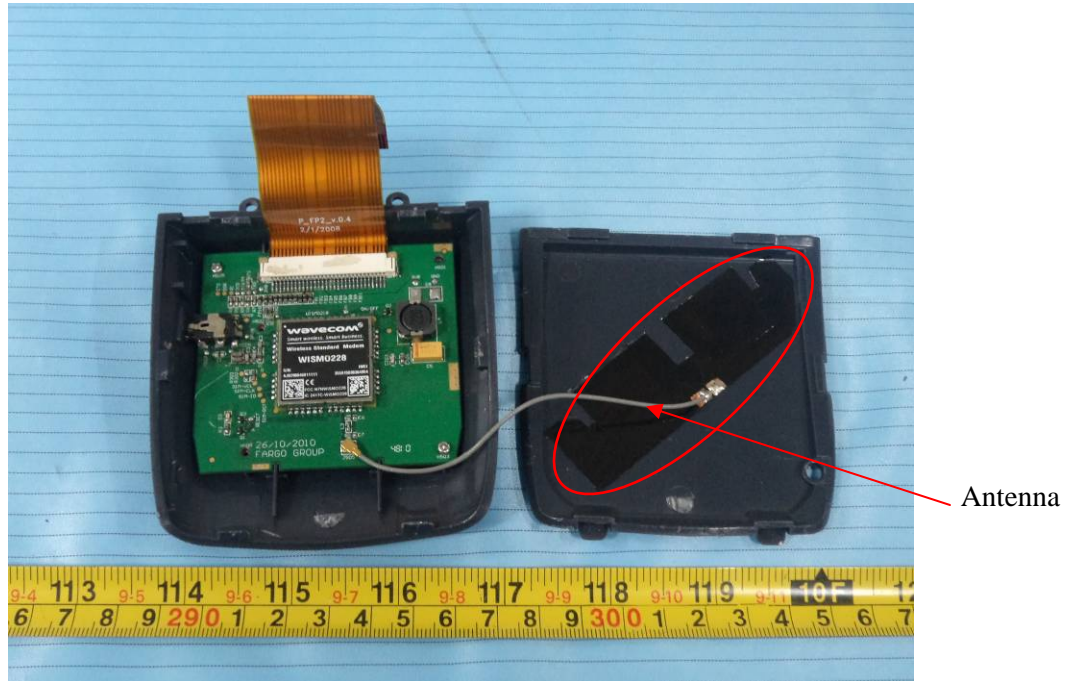
EUT – RF Module Cover off View
