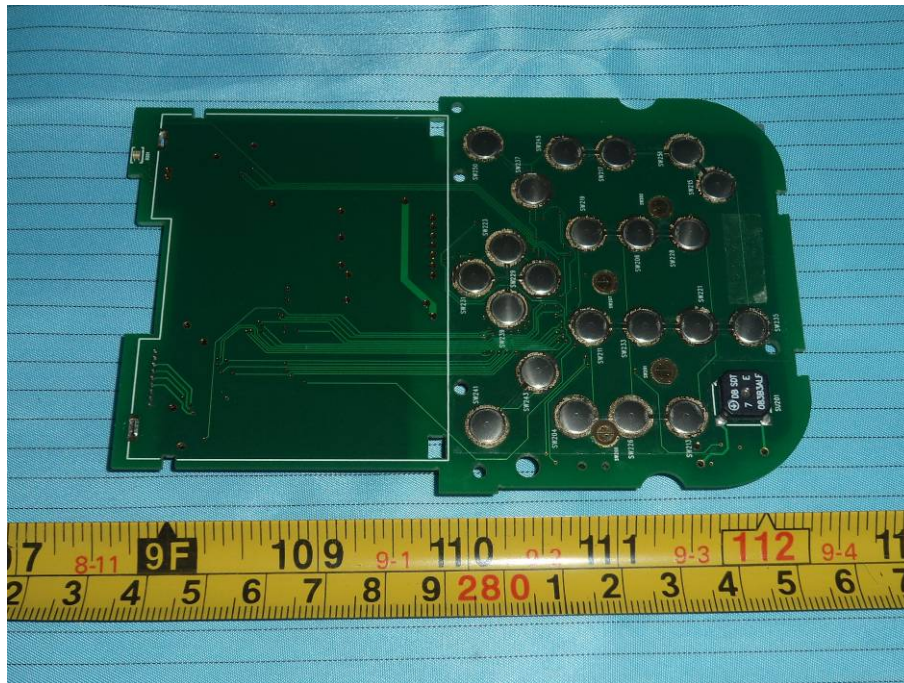
EUT – P_P2_v.0.10 Board Top View
