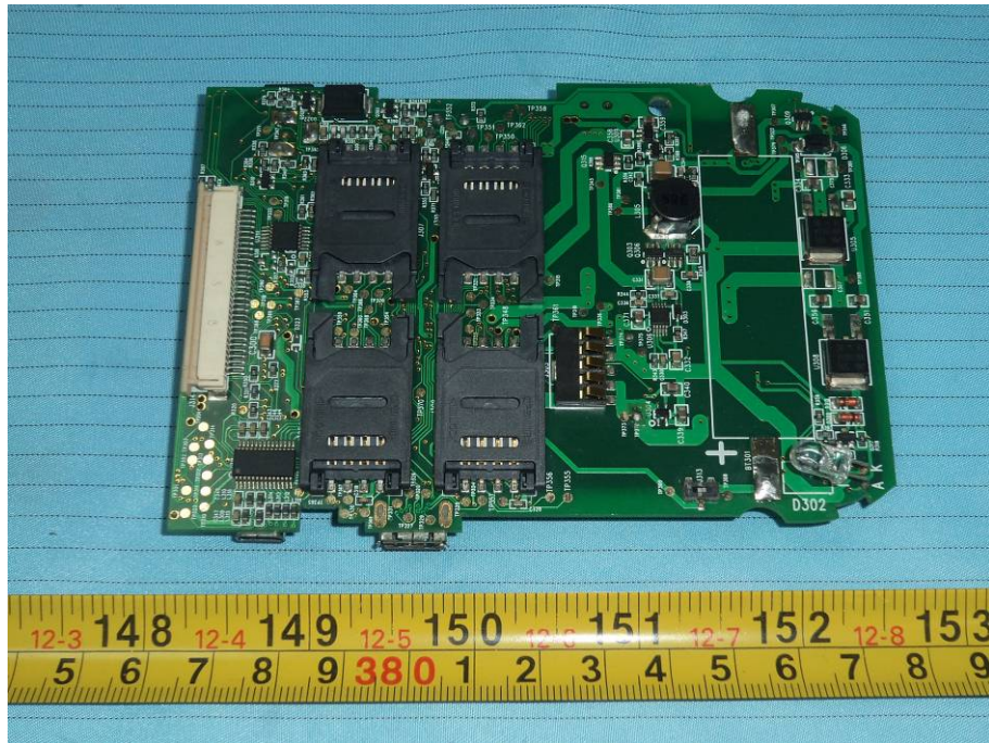
EUT – P P3_v.0.10 Board Top View
