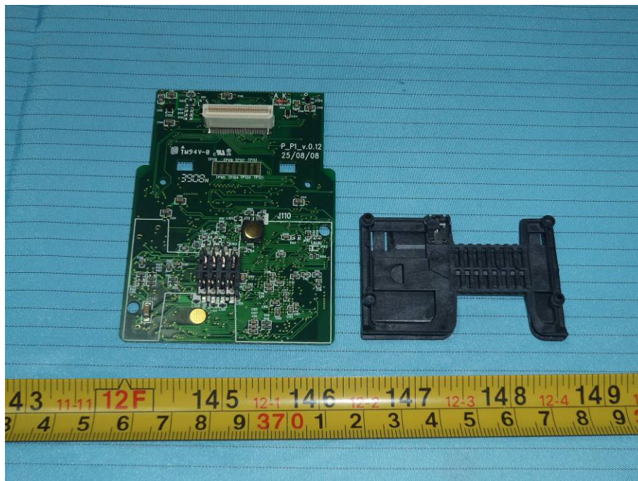
EUT – P_P1_v.0.12 Board Cover off Bottom View
