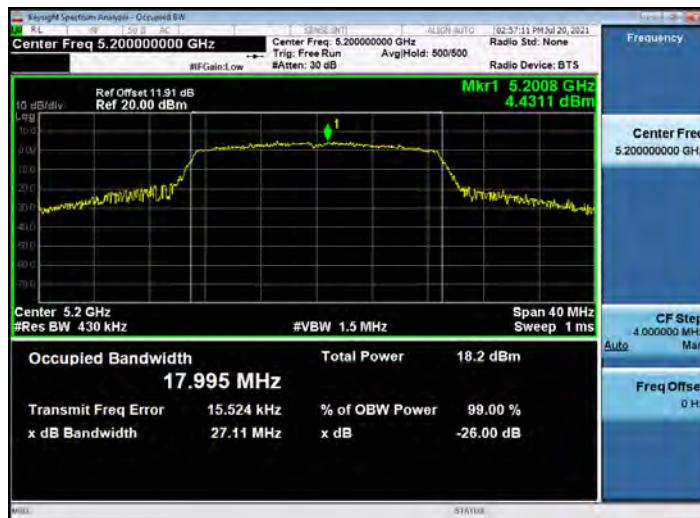
802.11n HT20_5200
