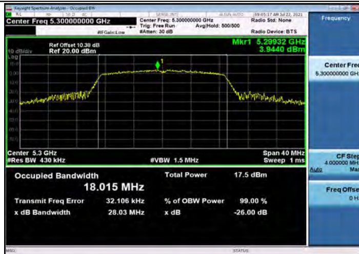
802.11n HT20_5300
