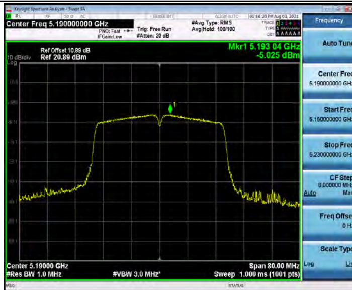
802.11n HT40_5190
