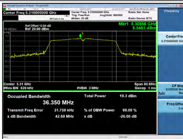
802.11ac VHT40_5310
