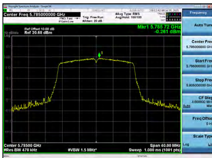
802.11n HT20_5785
