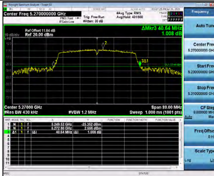
802.11n HT40_5270
