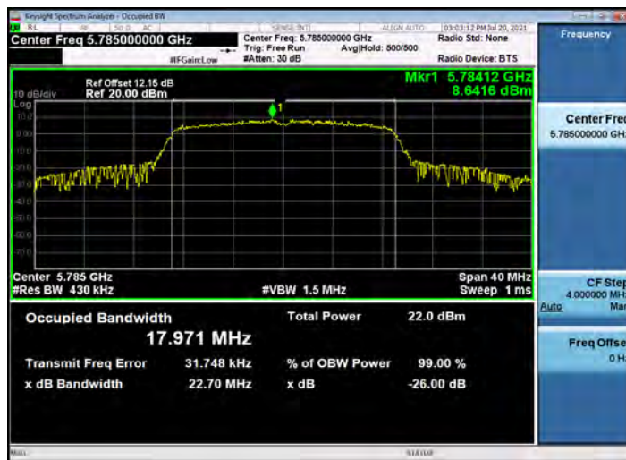
802.11n HT20_5785
