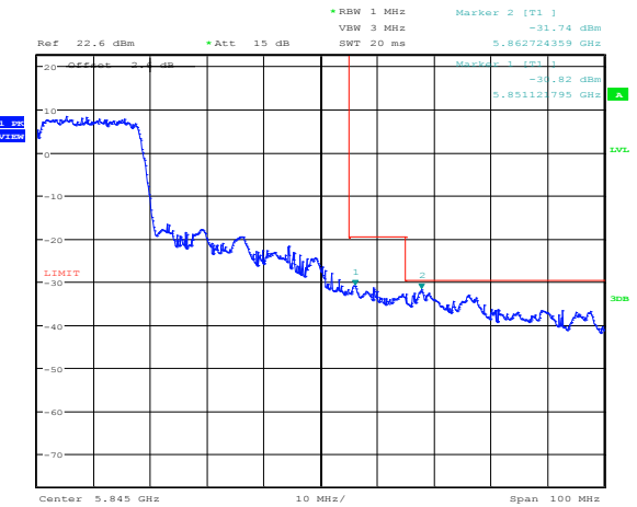
Figure 8.4-50: Upper band edge emission 802.11n HT20 with MCS 7
