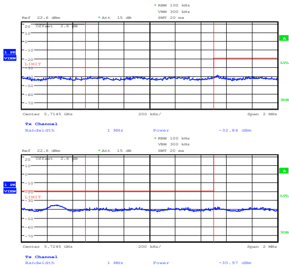
Figure 8.4-41: Lower band edges emissions for 802.11n HT40 with MCS 0
