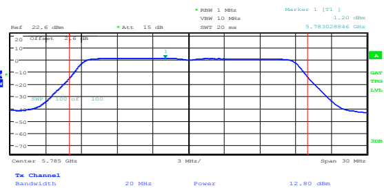
Figure 8.3-2: Sample plot for power and PSD on 802.11n HT20
