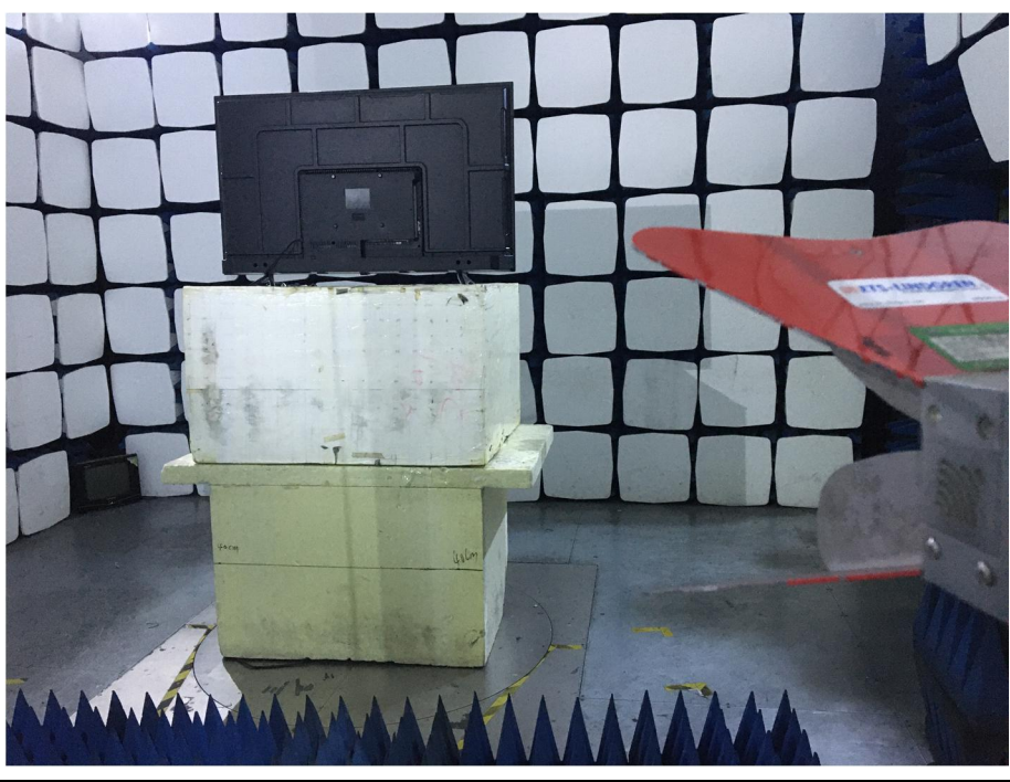
Radiation Emission Test Setup (1GHz to 18GHz)
