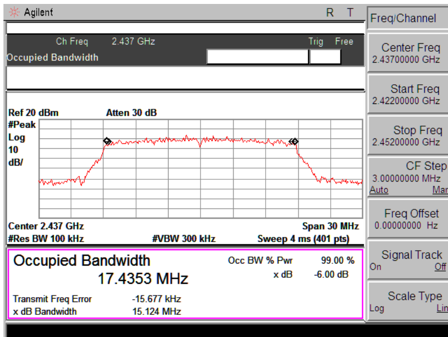
802.11n-HT20-Middle Channel
