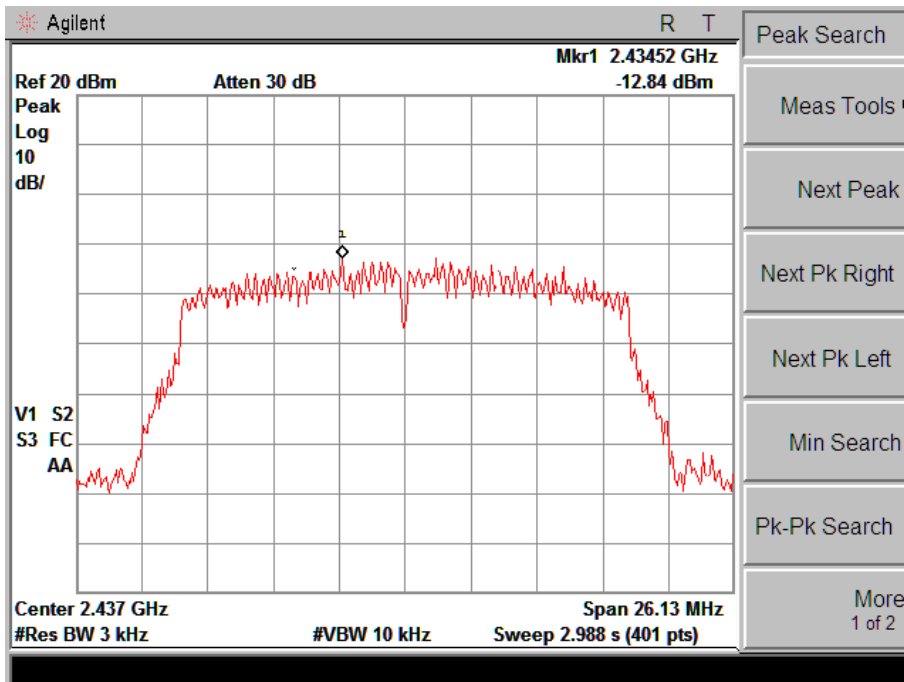
802.11n-HT20-Middle Channel
