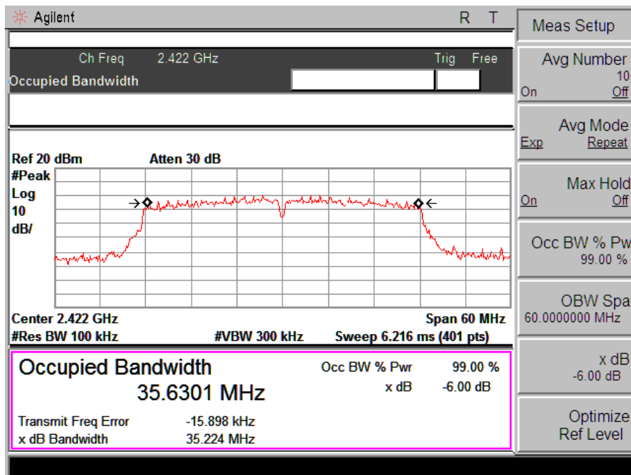
802.11n-HT40-Low Channel
