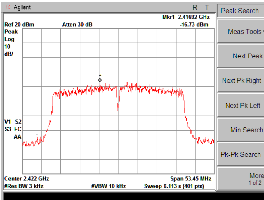
802.11n-HT40-Low Channel
