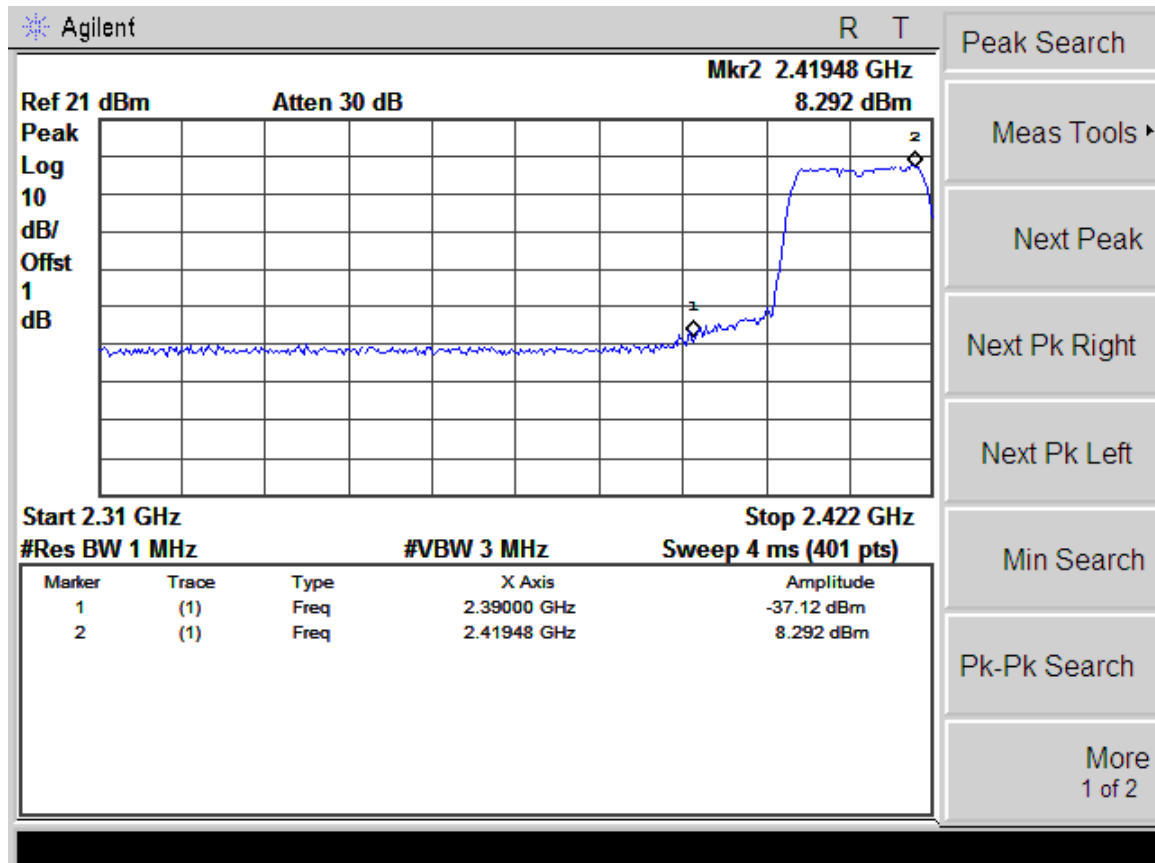
(Plot 4.5.3 A1: Channel 1: 2412MHz @ 802.11n(20MHz))
