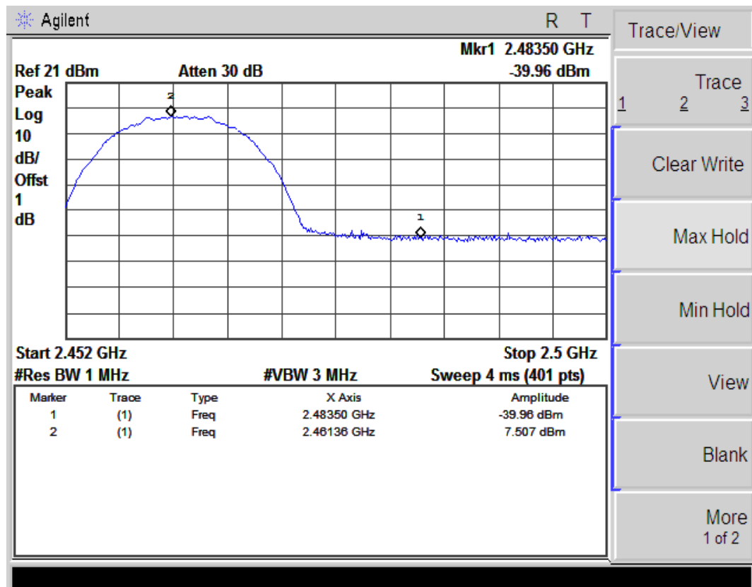
(Plot 4.5.1 A3: Channel 11: 2462MHz @ 802.11b)
