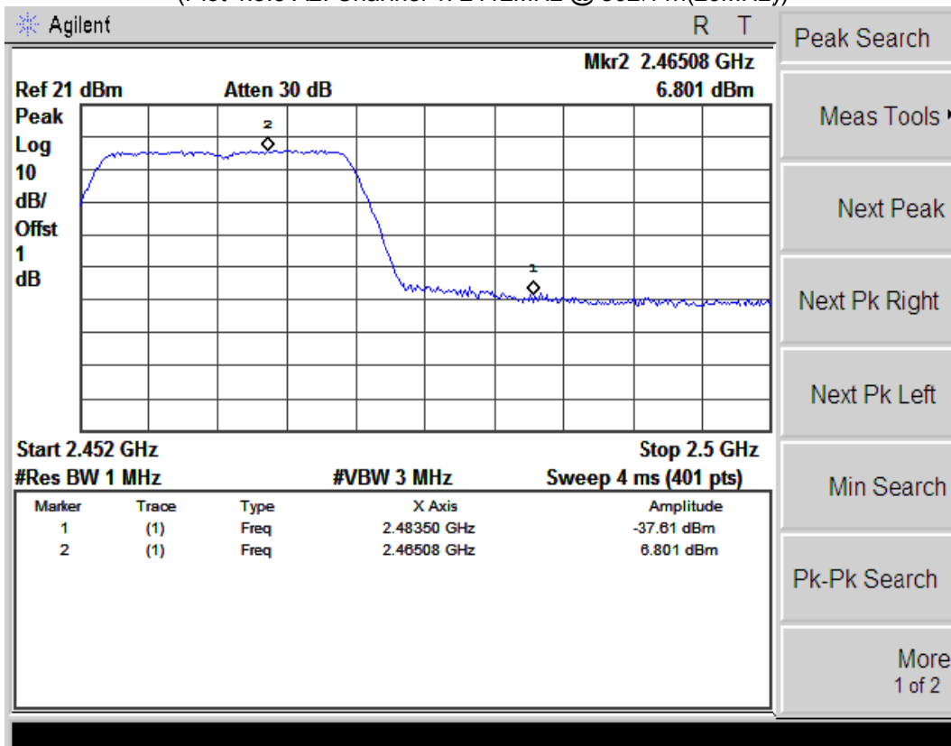
(Plot 4.5.3 A3: Channel 11: 2462MHz @ 802.11n(20MHz))
