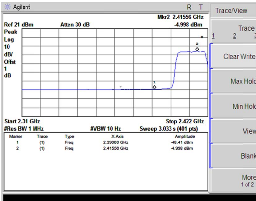
(Plot 4.5.2 A2: Channel 1: 2412MHz @ 802.11g)
