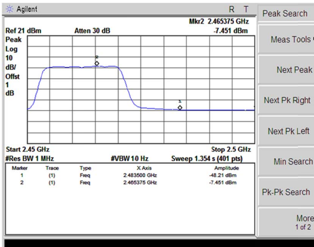
(Plot 4.5.2 A4: Channel 11: 2462MHz @ 802.11g)
