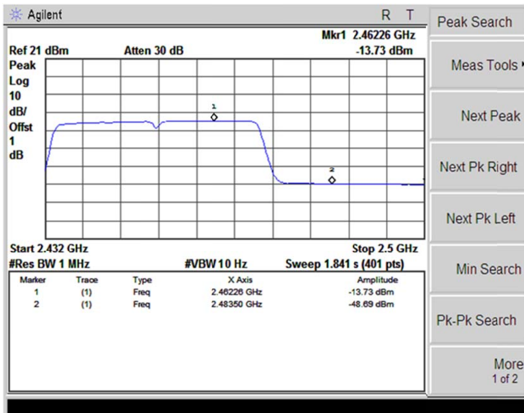
(Plot 4.5.3 A4: Channel 9: 2452MHz @ 802.11n(40MHz))
