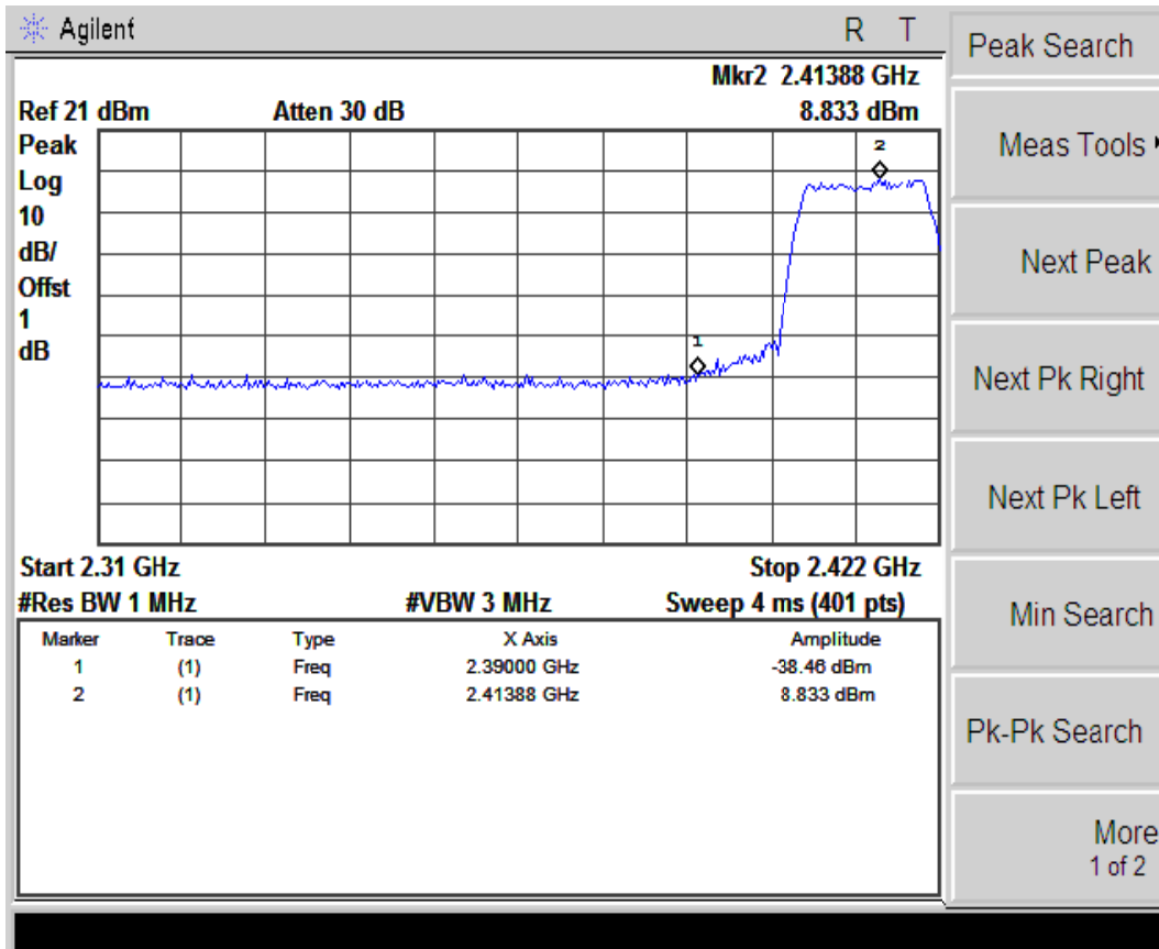
(Plot 4.5.2 A1: Channel 1: 2412MHz @ 802.11g)
