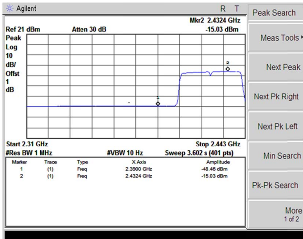
(Plot 4.5.3 A2: Channel 3: 2422MHz @ 802.11n(40MHz))
