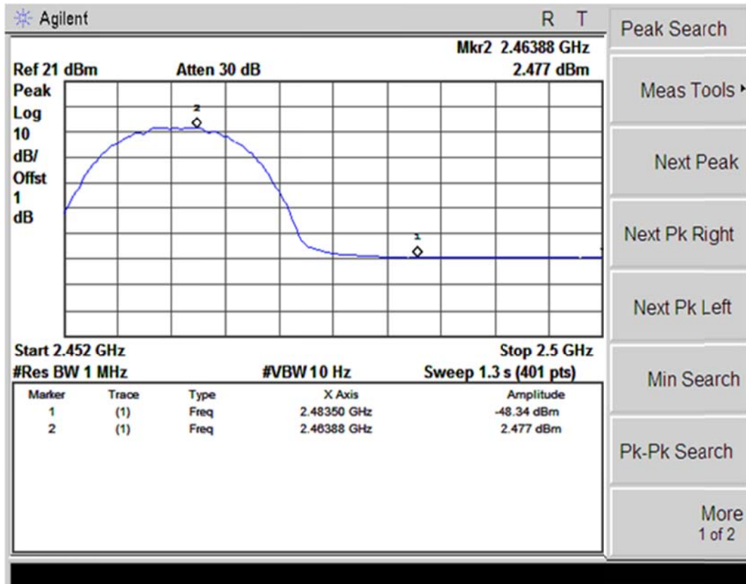
(Plot 4.5.1 A4: Channel 11: 2462MHz @ 802.11b)
