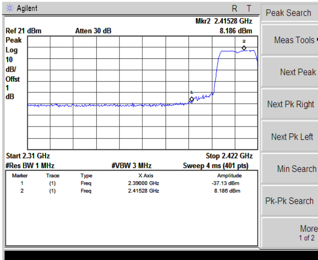
(Plot 4.5.3 A1: Channel 1: 2412MHz @ 802.11n(20MHz))
