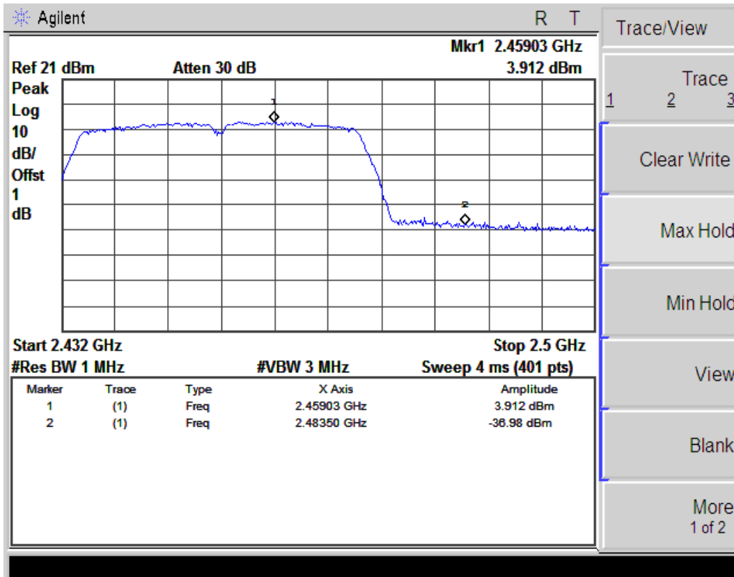
(Plot 4.5.3 A3: Channel 9: 2452MHz @ 802.11n(40MHz))
