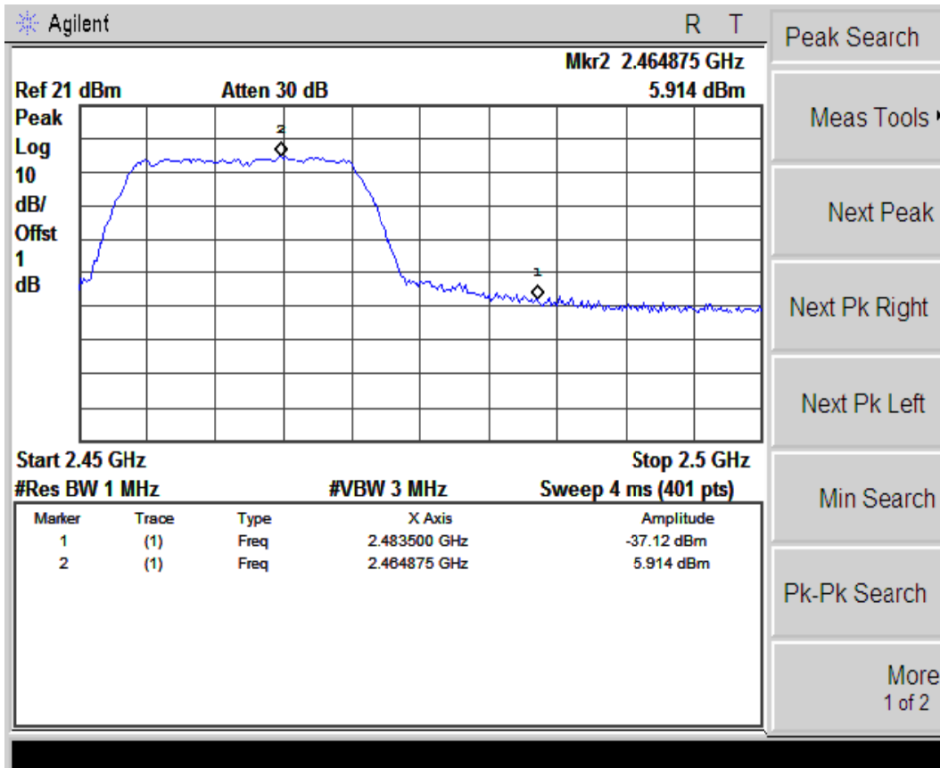
(Plot 4.5.2 A3: Channel 11: 2462MHz @ 802.11g)
