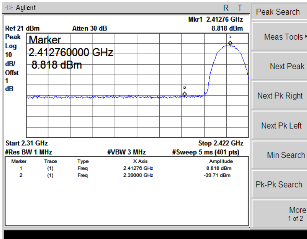
(Plot 4.5.1 A1: Channel 1: 2412MHz @ 802.11b)
