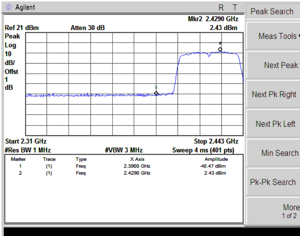
(Plot 4.5.3 A1: Channel 3: 2422MHz @ 802.11n(40MHz))
