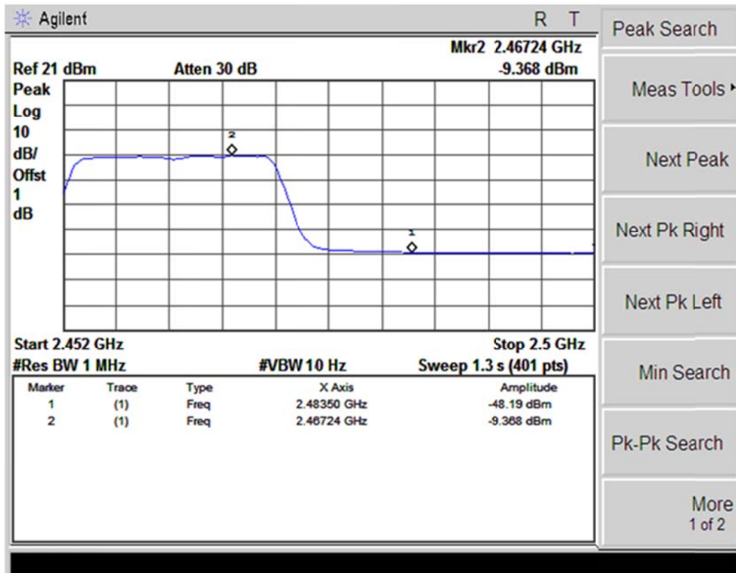
(Plot 4.5.3 A4: Channel 11: 2462MHz @ 802.11n(20MHz))
