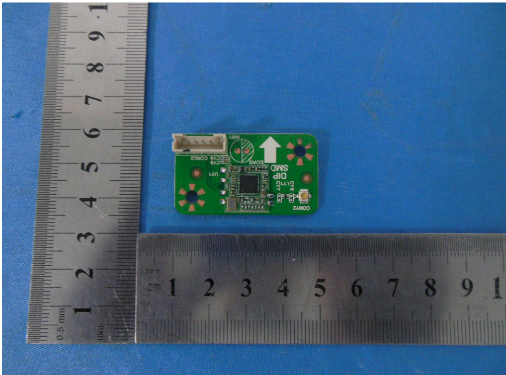
EUT –PCB WIFI View
