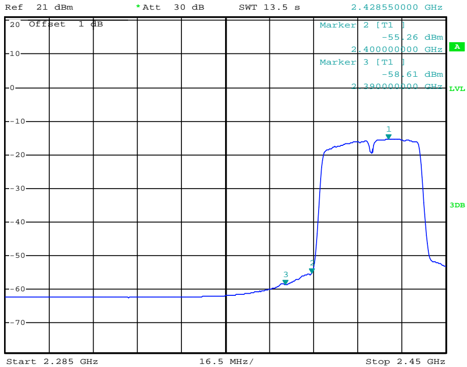
(Plot 4.5.3 A1: Channel 3: 2422MHz @ 802.11n(40MHz))
