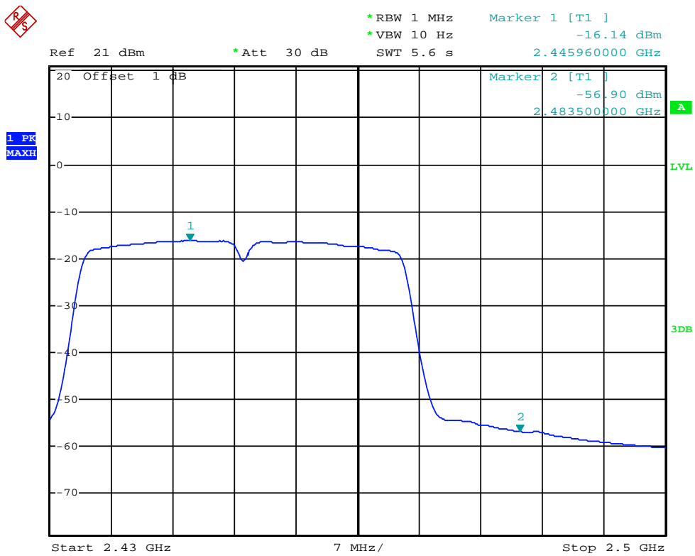
(Plot 4.5.3 A3: Channel 9: 2452MHz @ 802.11n(40MHz))
