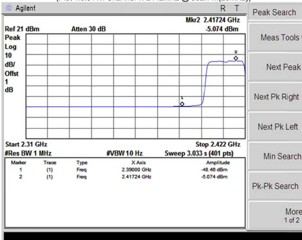
(Plot 4.5.3 A1: Channel 1: 2412MHz @ 802.11n(20MHz))
