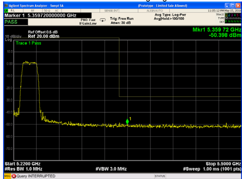
802.11a U-NII-1 Band edge-right side
