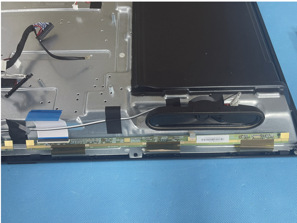
EUT Housing and Board View 3
