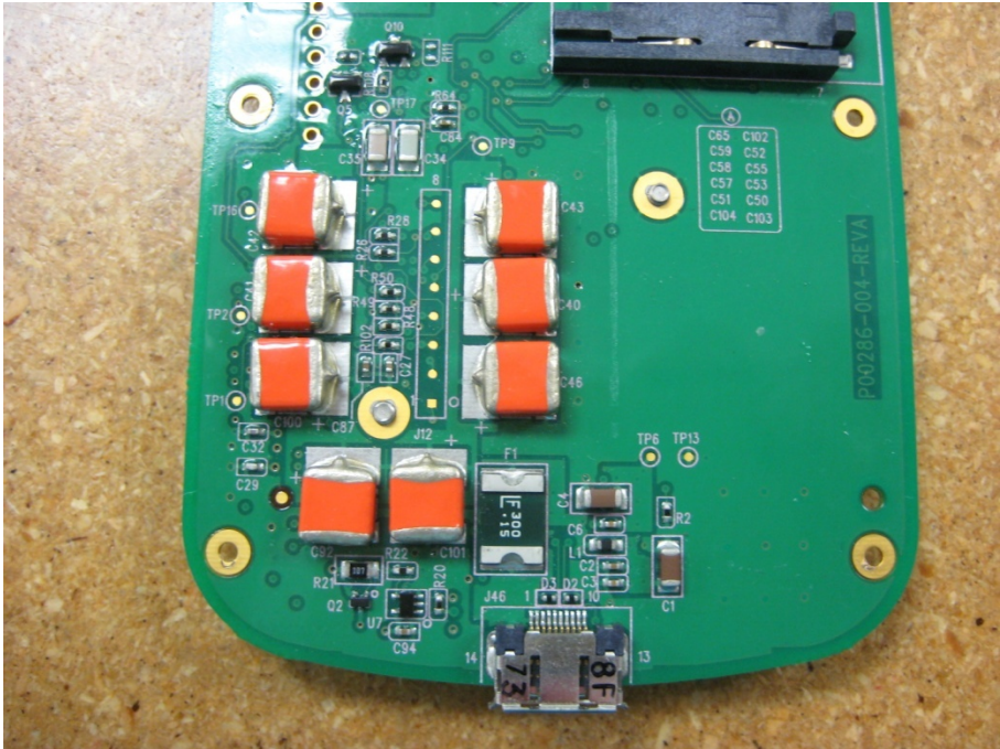
Main board back side close-up 2
