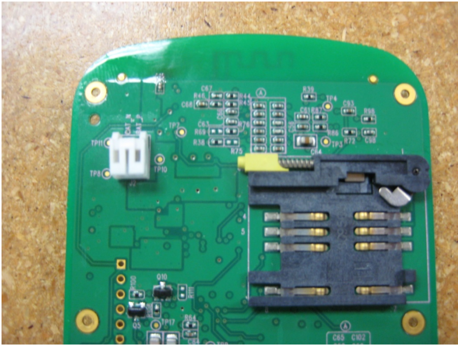
Main board back side close-up 1
