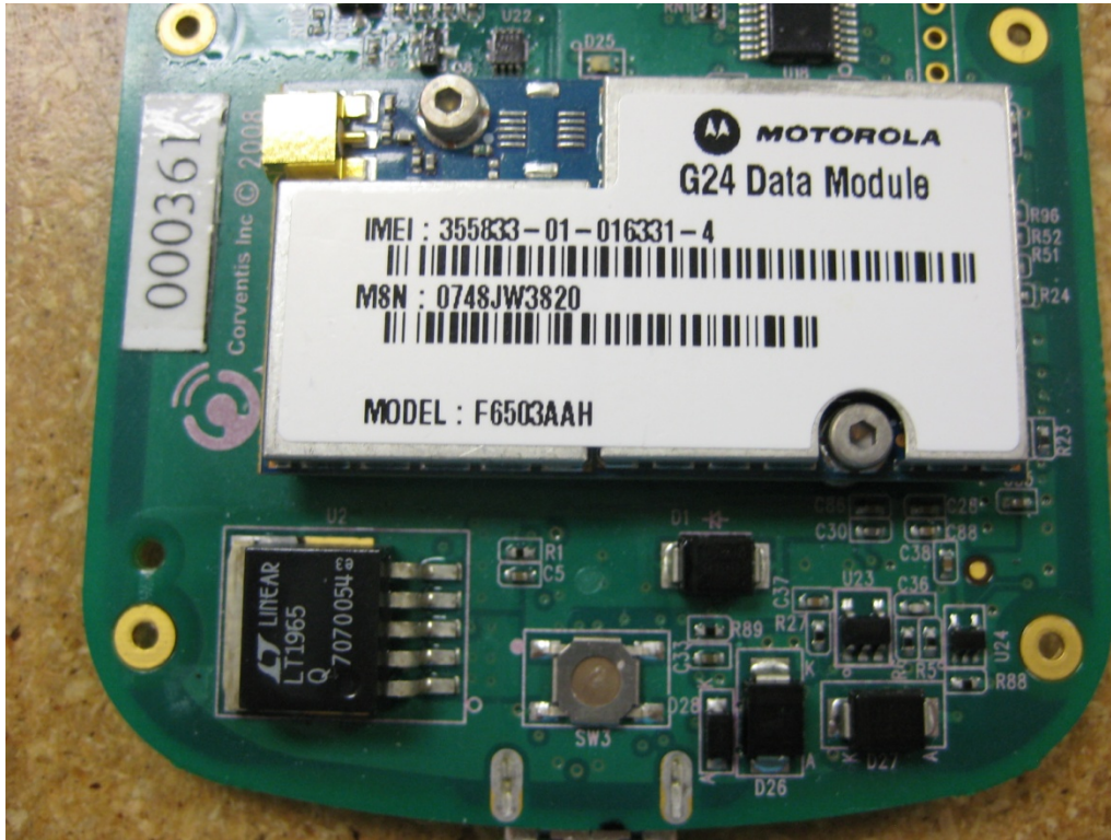
Main Board Top View Close-up 2
