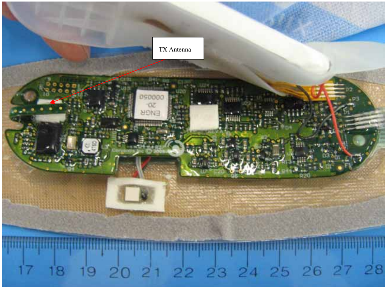
Figure 1: Internal photo of PiiX – PCB Component Side
