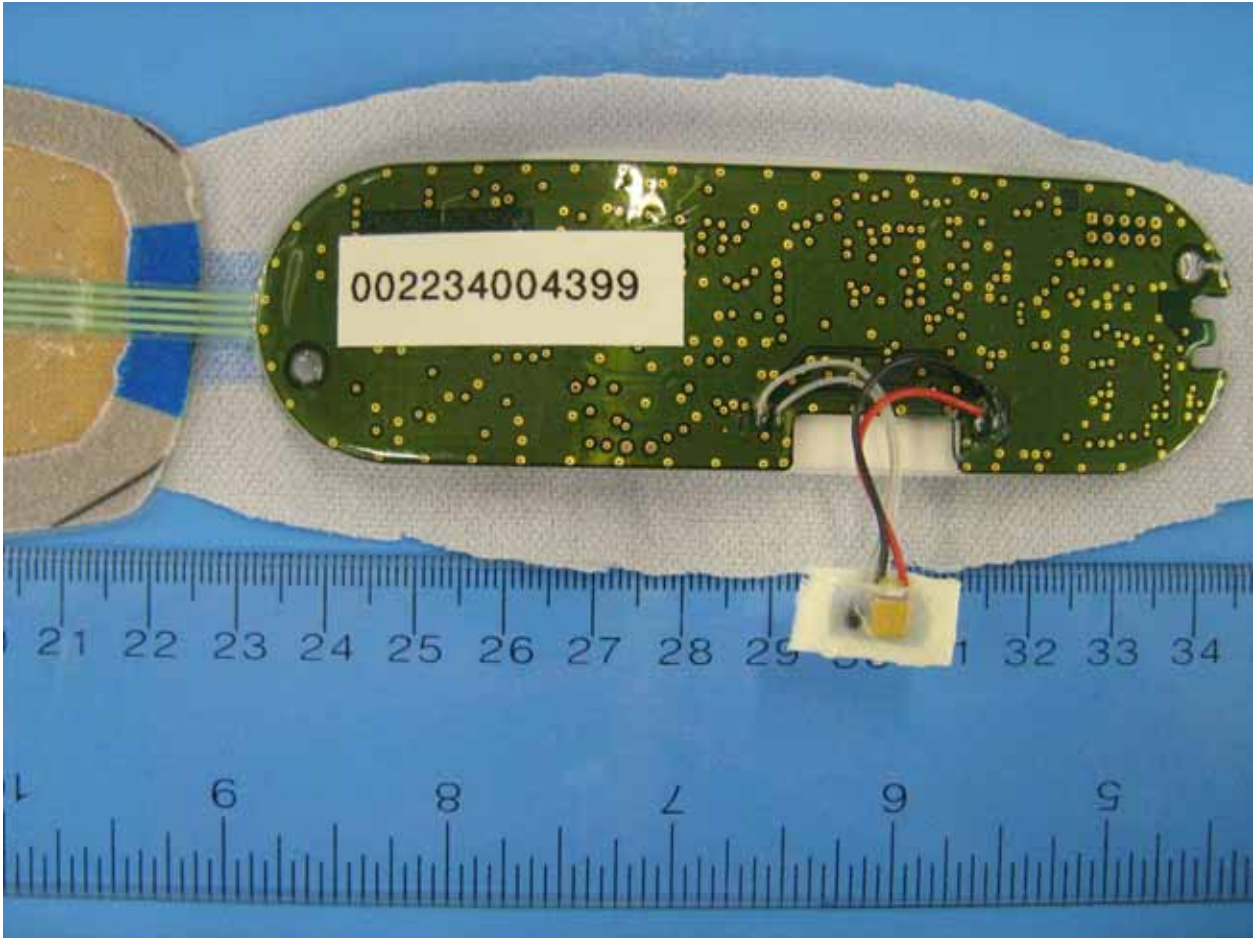
Figure 2: Internal photo of PiiX – PCB Soldered Side
