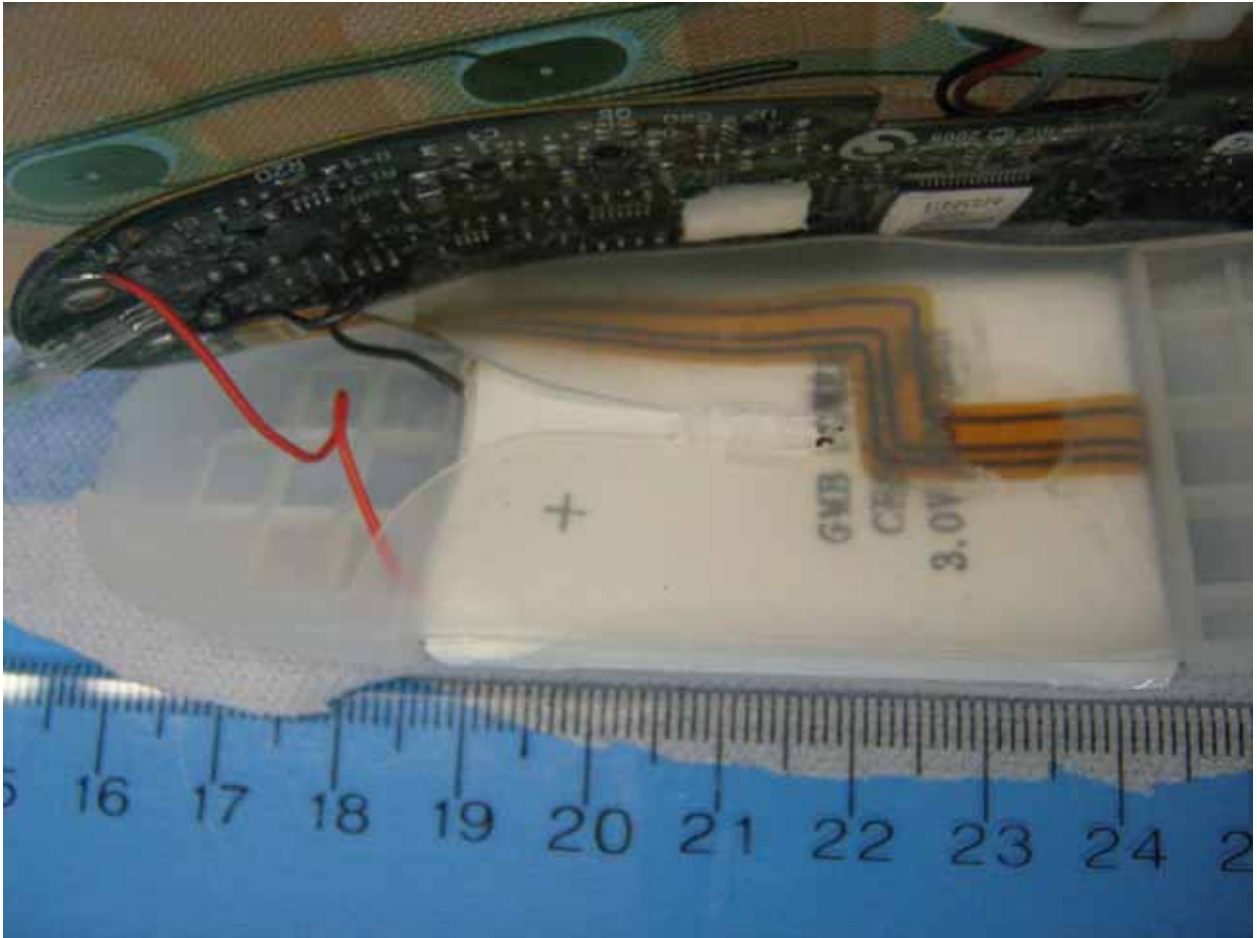
Figure 3: Internal photo of PiiX – Battery
