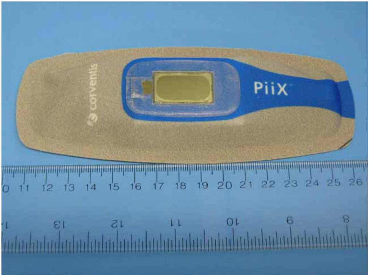
Figure 1: External Photo of Piix – Top View
