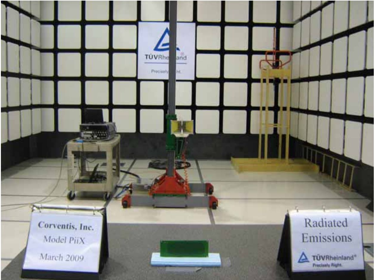
Figure 4: Photo of Test Setup for PiiX, 1GHz to 18GHz (Rear View)
