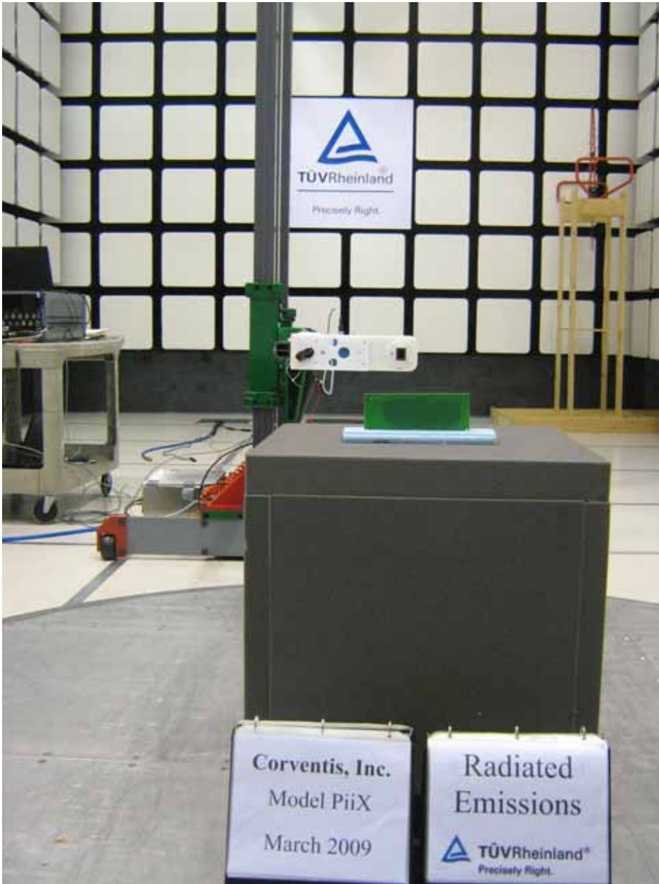
Figure 6: Photo of Test Setup for PiiX, 18 GHz to 26GHz (Rear View)
