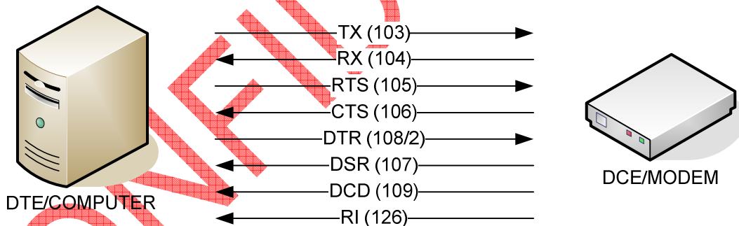
Figure 6-7-1: DTE-DCE RS232 interface
