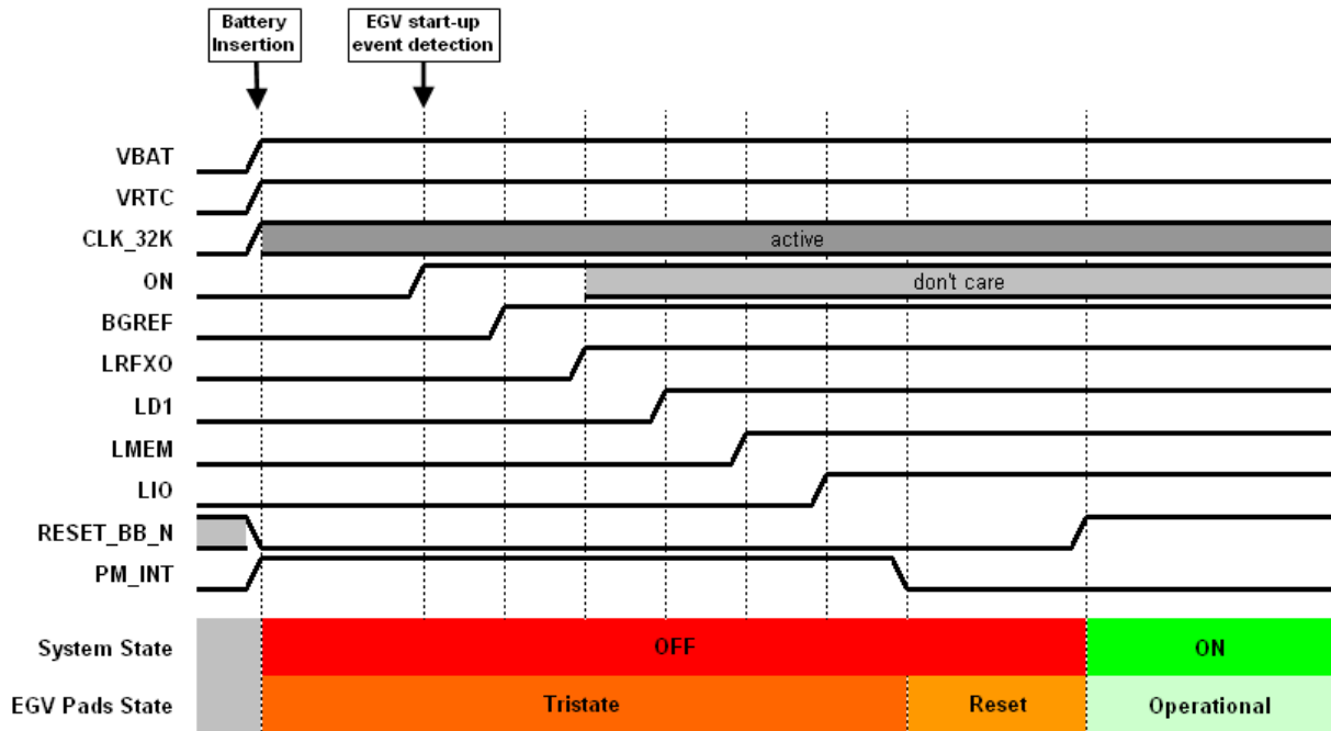
Figure 6-2-1: Power on sequence
