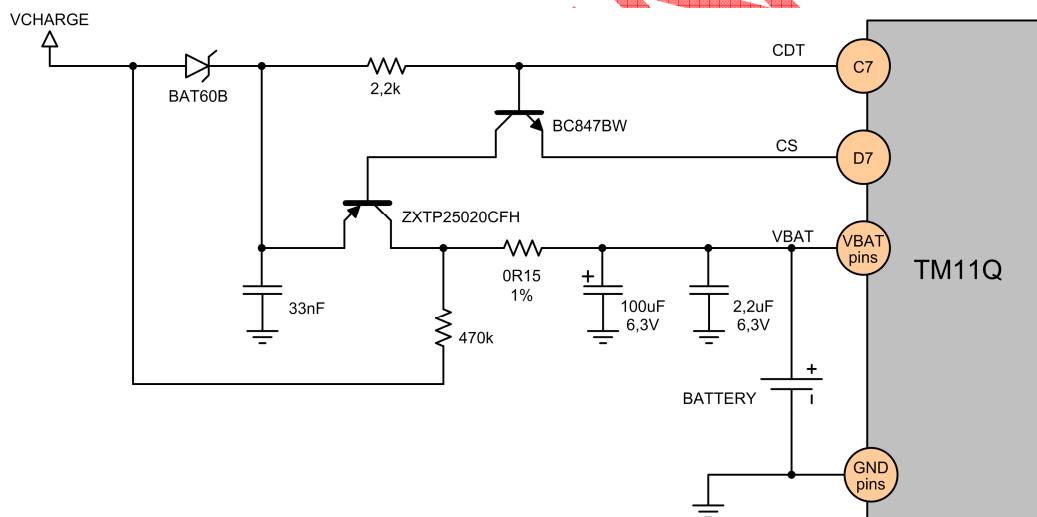
Figure 5-2-2: Charger circuit description
