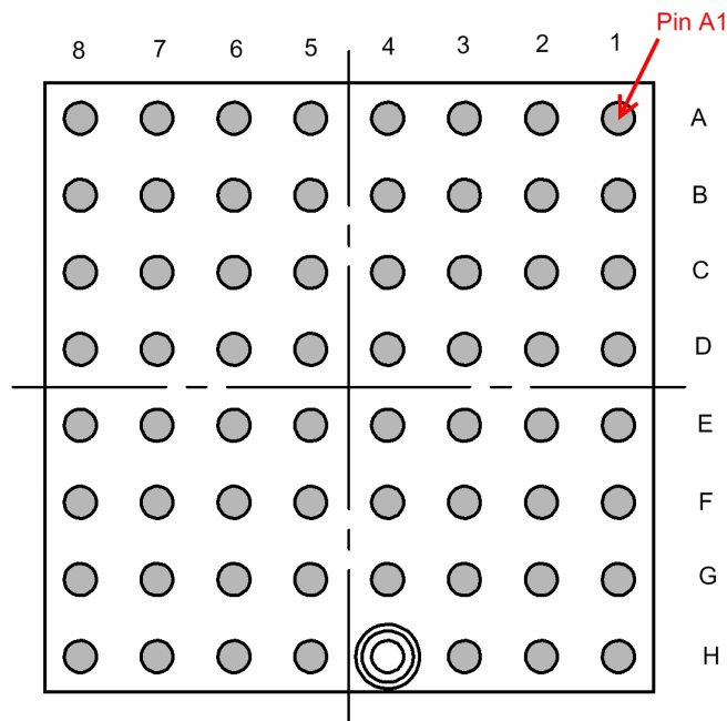
Figure 6-1: Module BGA pins
