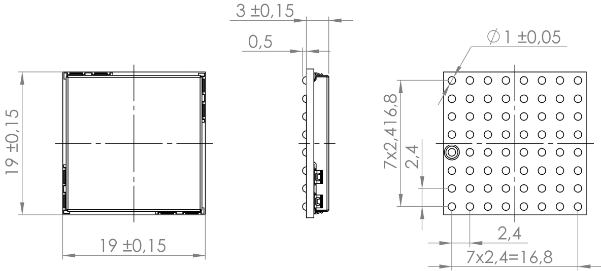
Figure 5-3-1: TM11Q module
