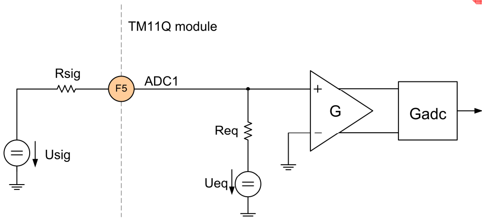
Figure 6-11-1: Equivalent network for ADC single-ended measurement
