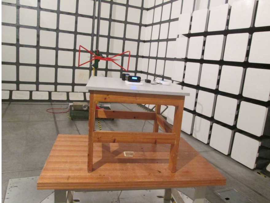
Transmitting Radiated Emissions (Below 1 GHz)
